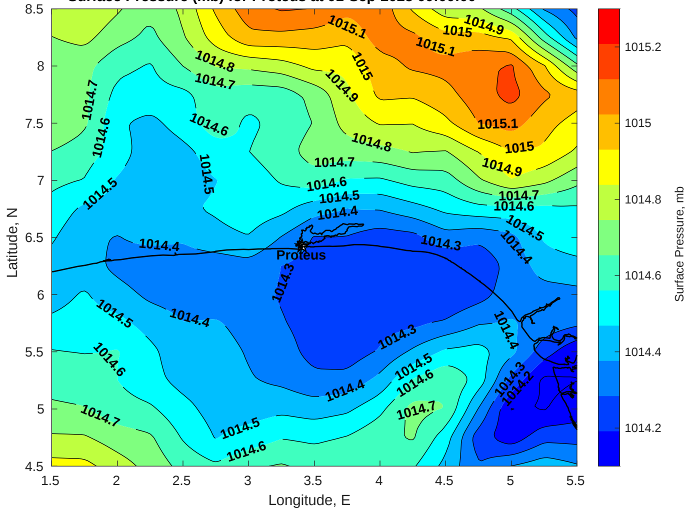
Surface Pressure (mb) for Proteus at 01-Sep-2025 00:00:00
