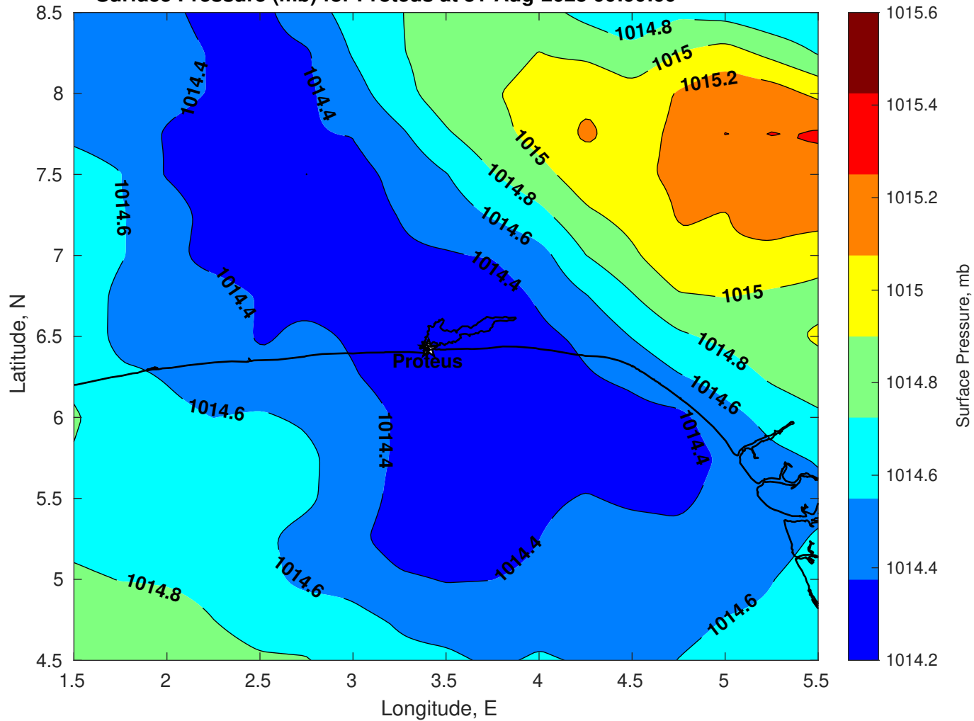
Surface Pressure (mb) for Proteus at 31-Aug-2025 00:00:00
