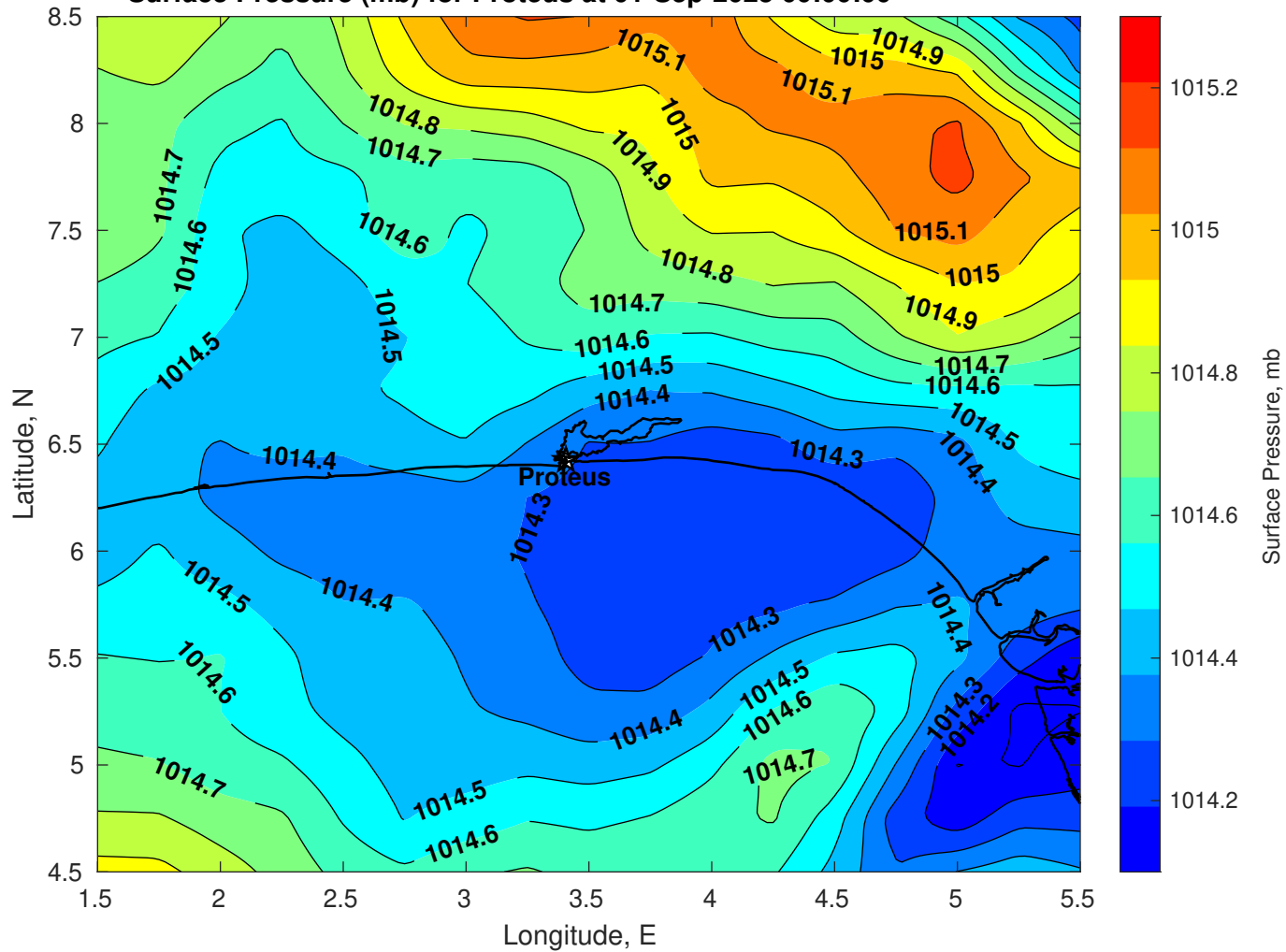
Surface Pressure (mb) for Proteus at 01-Sep-2025 00:00:00
