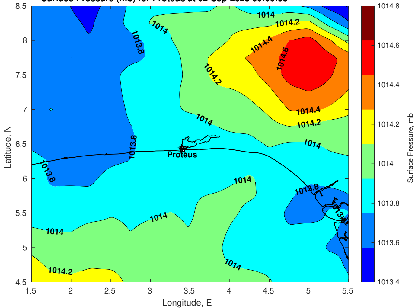
Surface Pressure (mb) for Proteus at 02-Sep-2025 00:00:00
