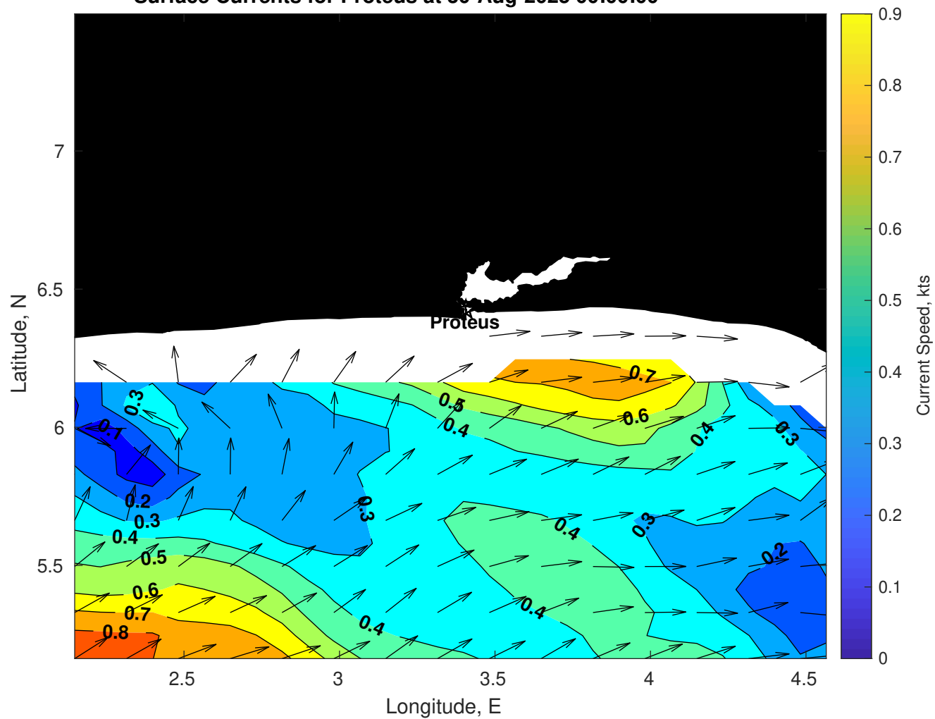
Surface Currents for Proteus at 30-Aug-2025 00:00:00
