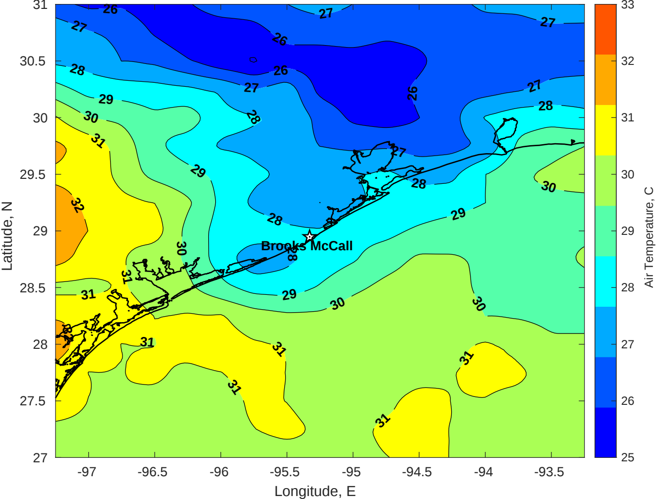
Air Temperature (C) for Brooks McCall at 15-Sep-2025
