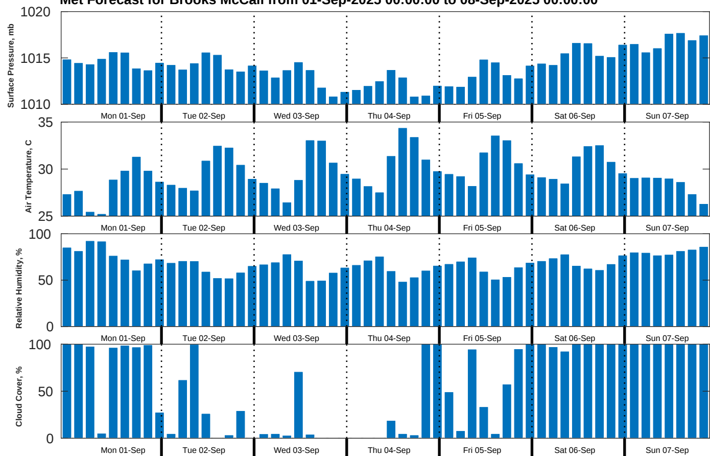
Met Forecast for Brooks McCall from 01-Sep-2025 00:00:00 to 08-Sep-2025 00:00:00
