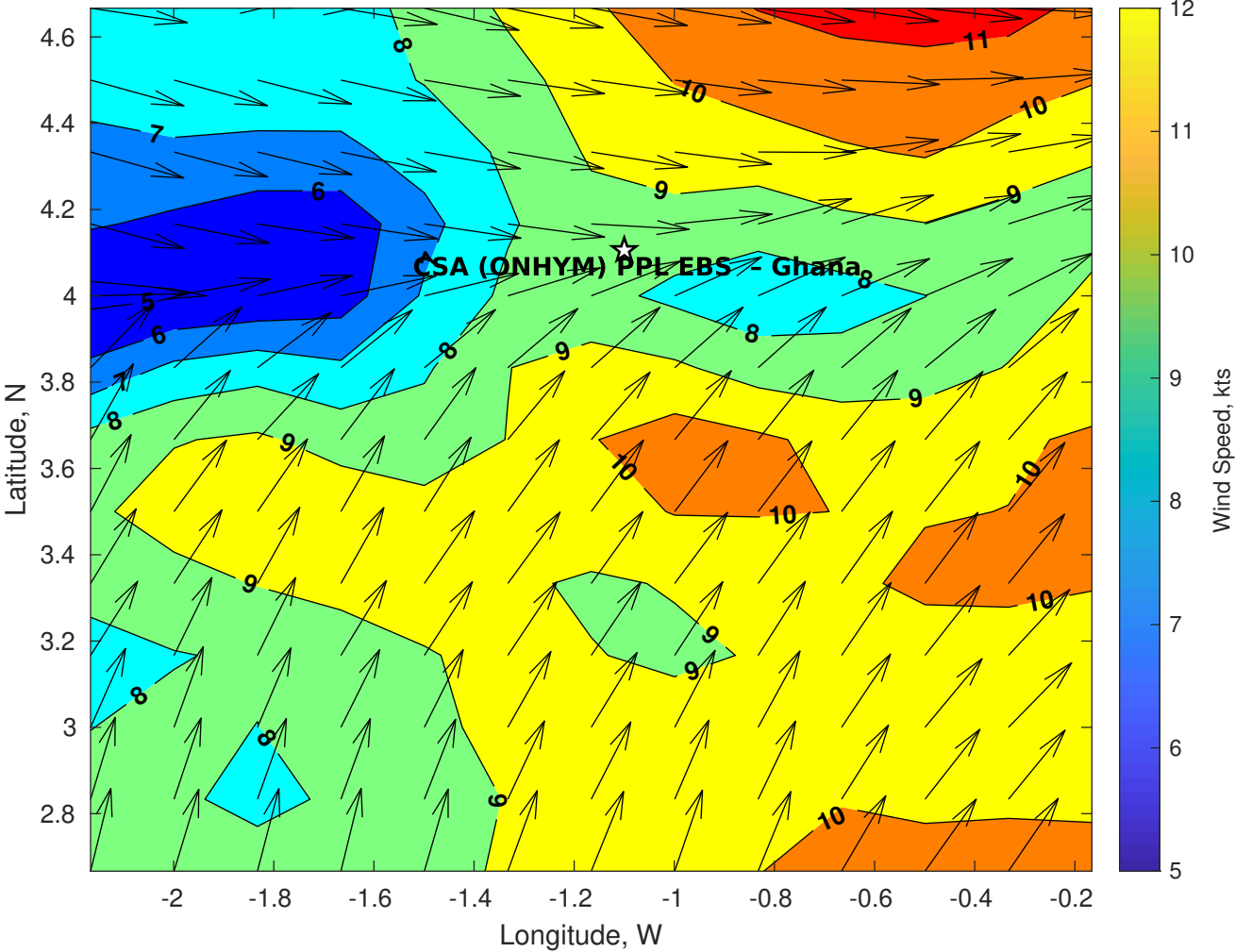
Winds (kts) for CSA (ONHYM) PPL EBS - Ghana at 15-Sep-2025 09:00:00
