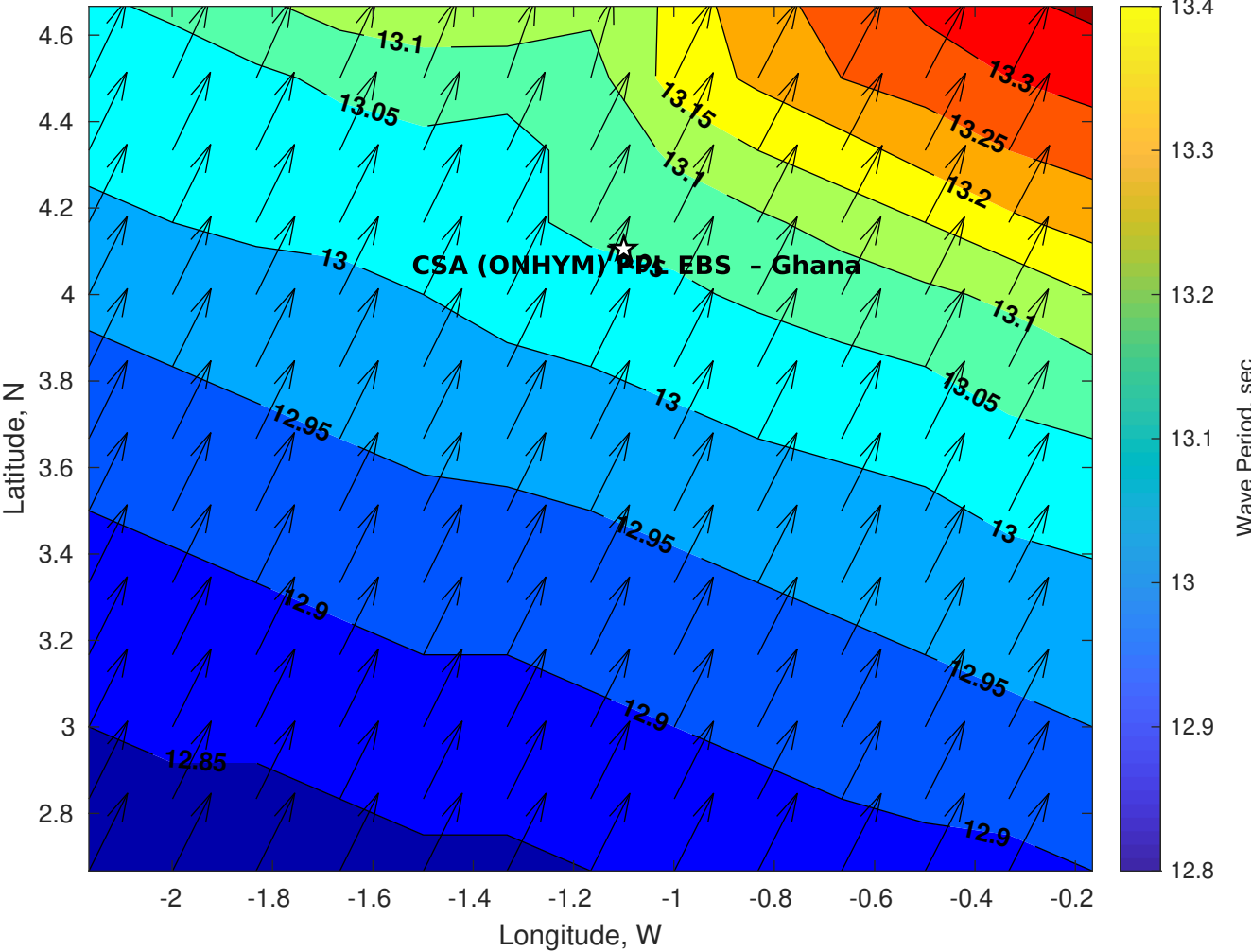
Wave Period (sec) for CSA (ONHYM) PPL EBS - Ghana at 15-Sep-2025 09:00:00
