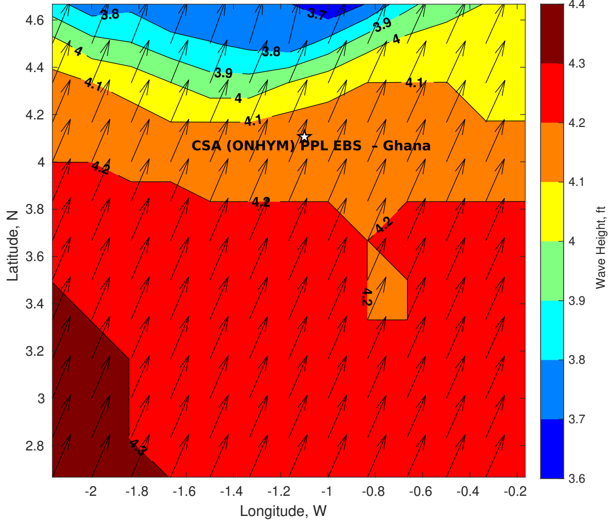
Wave Height (ft) for CSA (ONHYM) PPL EBS - Ghana at 15-Sep-2025 09:00:00
