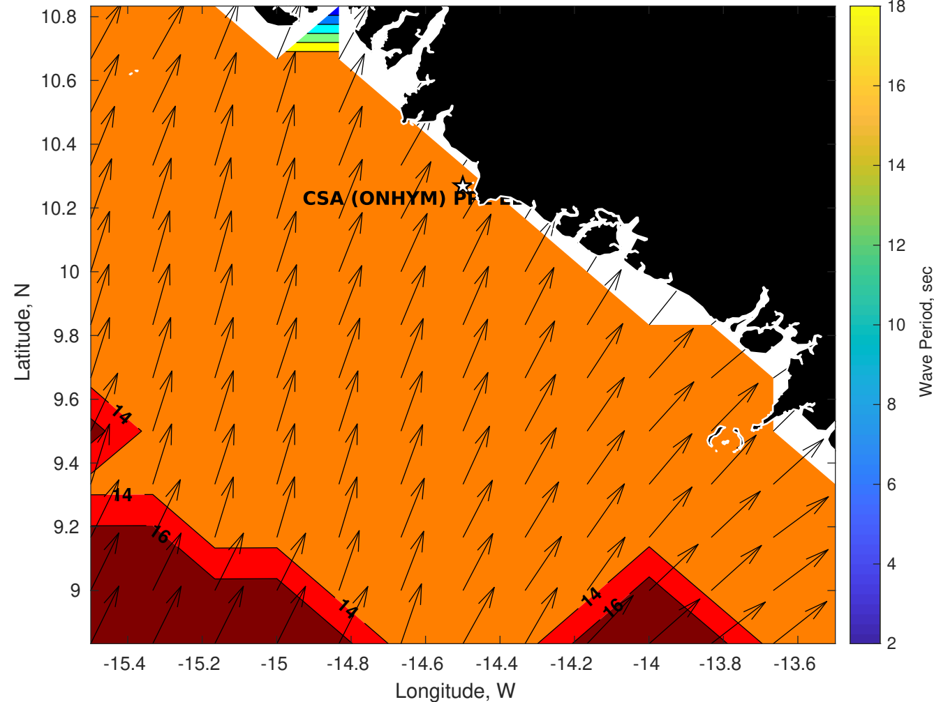
Wave Period (sec) for CSA (ONHYM) PPL EBS - Guinea at 15-Sep-2025 09:00:00
