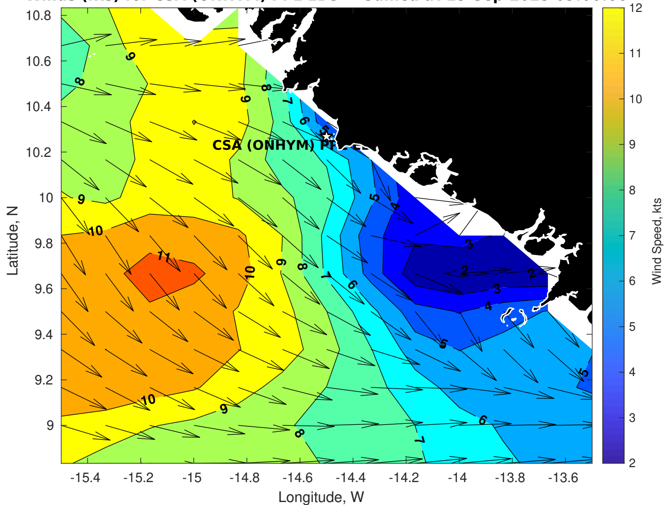
Winds (kts) for CSA (ONHYM) PPL EBS - Guinea at 15-Sep-2025 09:00:00
