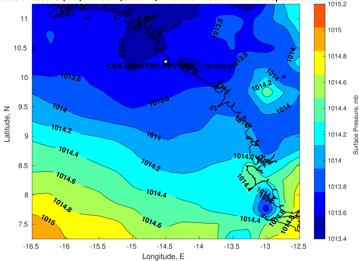
Surface Pressure (mb) for CSA (ONHYM) PPL EBS - Guinea at 15-Sep-2025 12:00:00
