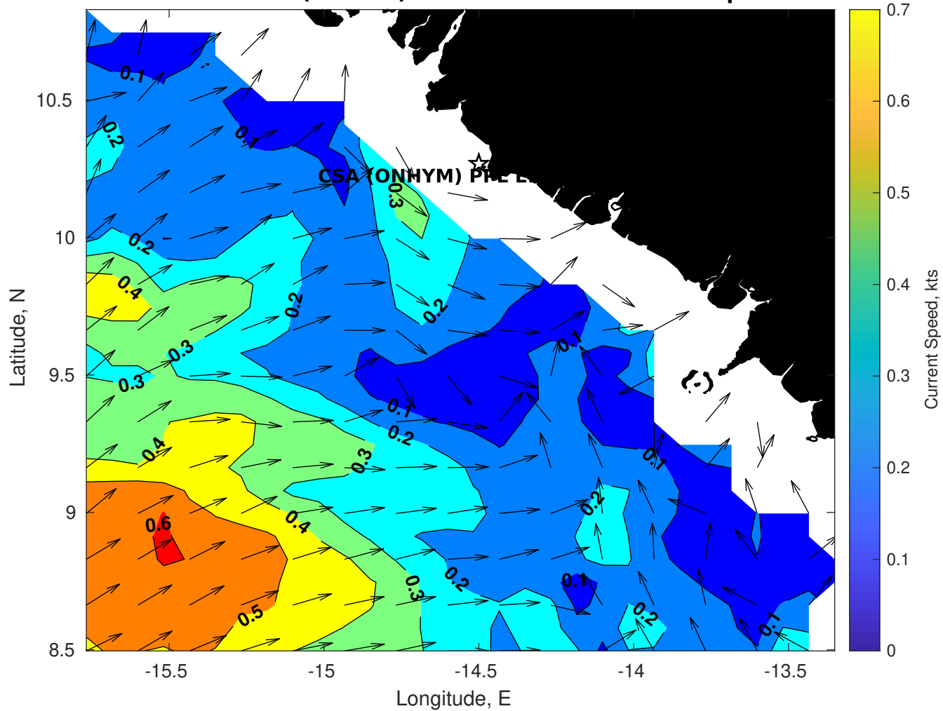
Surface Currents for CSA (ONHYM) PPL EBS - Guinea at 14-Sep-2025 00:00:00
