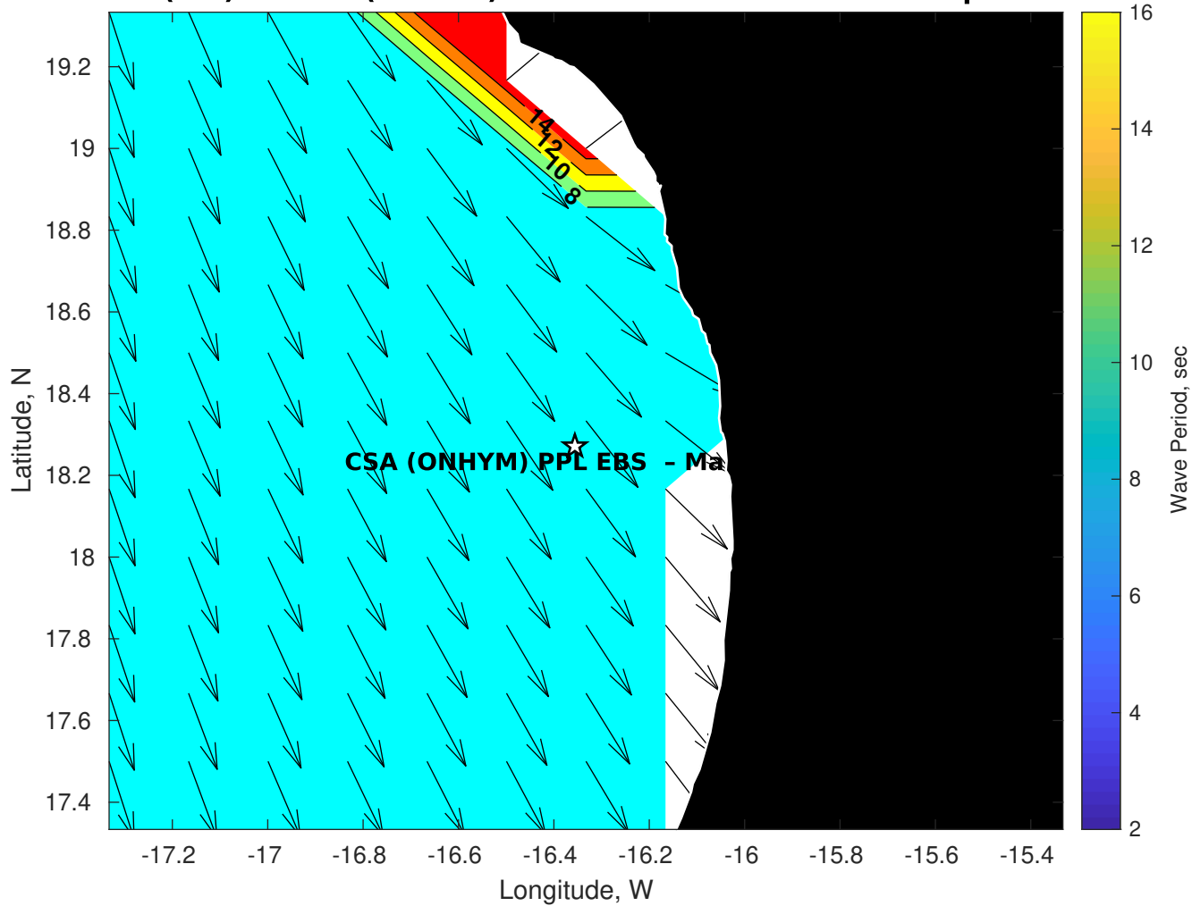
Wave Period (sec) for CSA (ONHYM) PPL EBS - Mauritania at 15-Sep-2025 09:00:00
