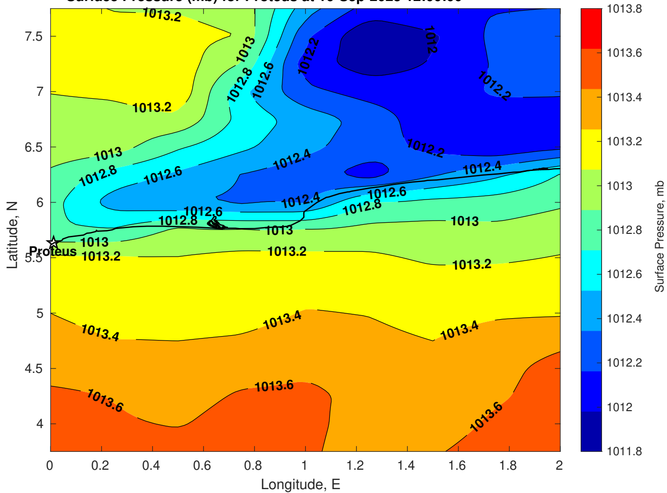
Surface Pressure (mb) for Proteus at 16-Sep-2025 12:00:00
