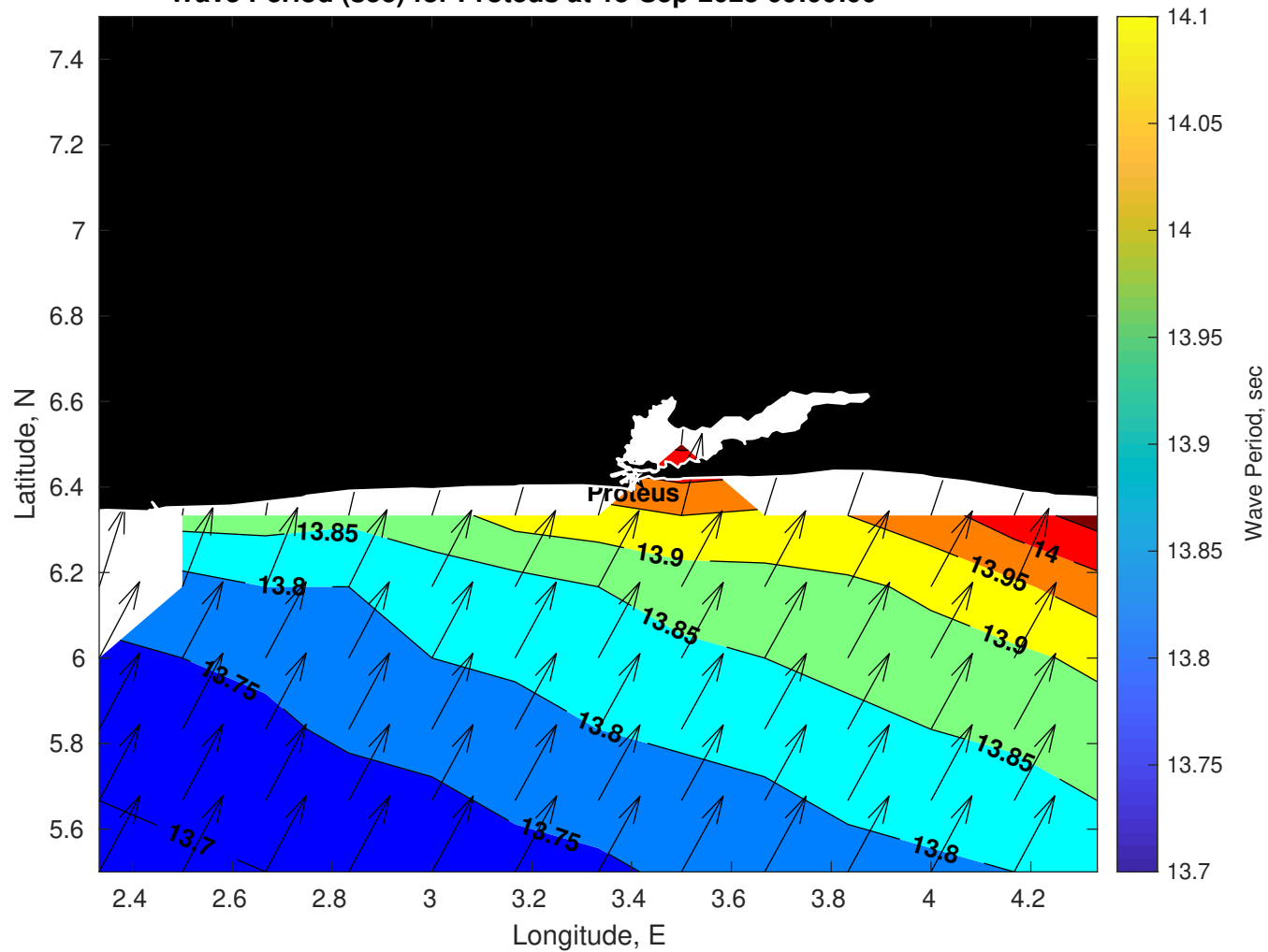
Wave Period (sec) for Proteus at 15-Sep-2025 09:00:00
