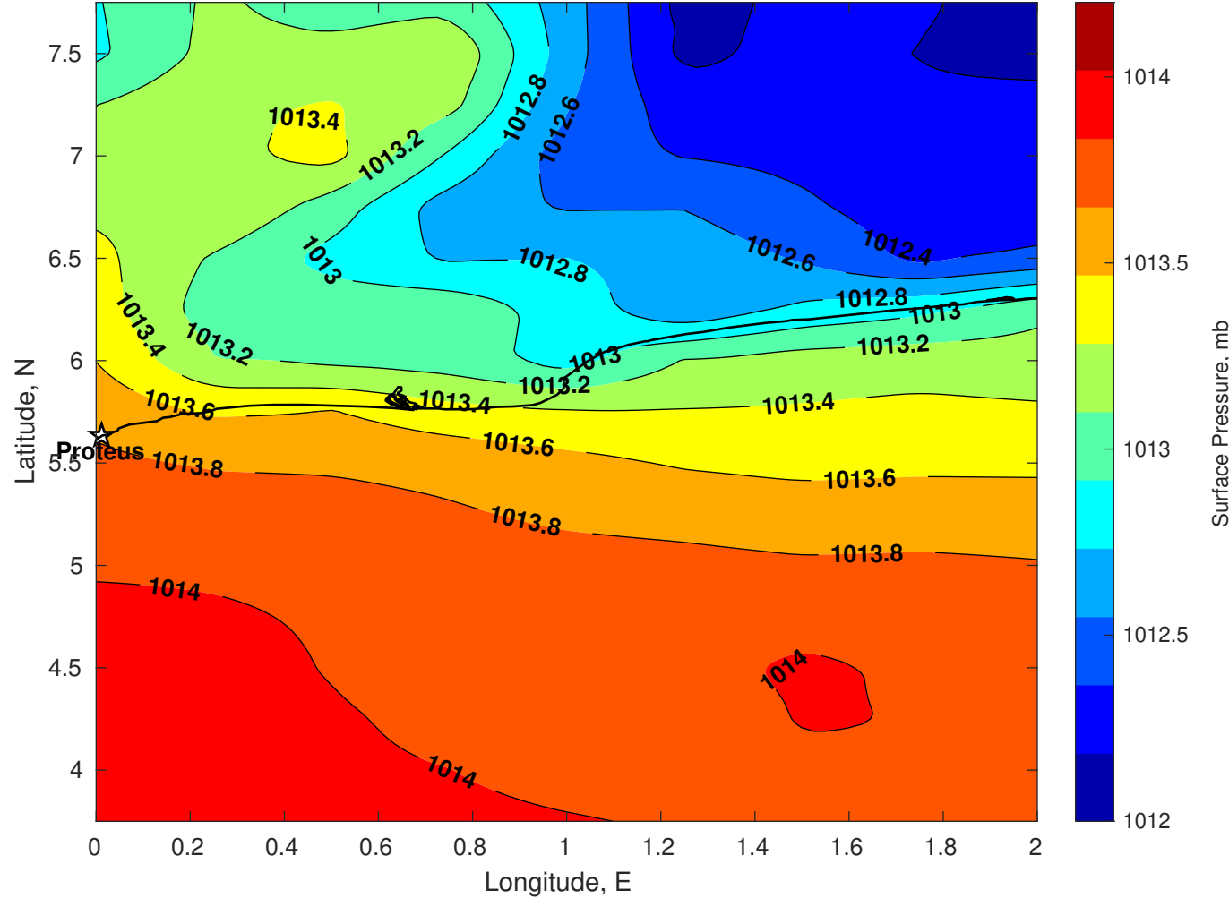
Surface Pressure (mb) for Proteus at 15-Sep-2025 12:00:00
