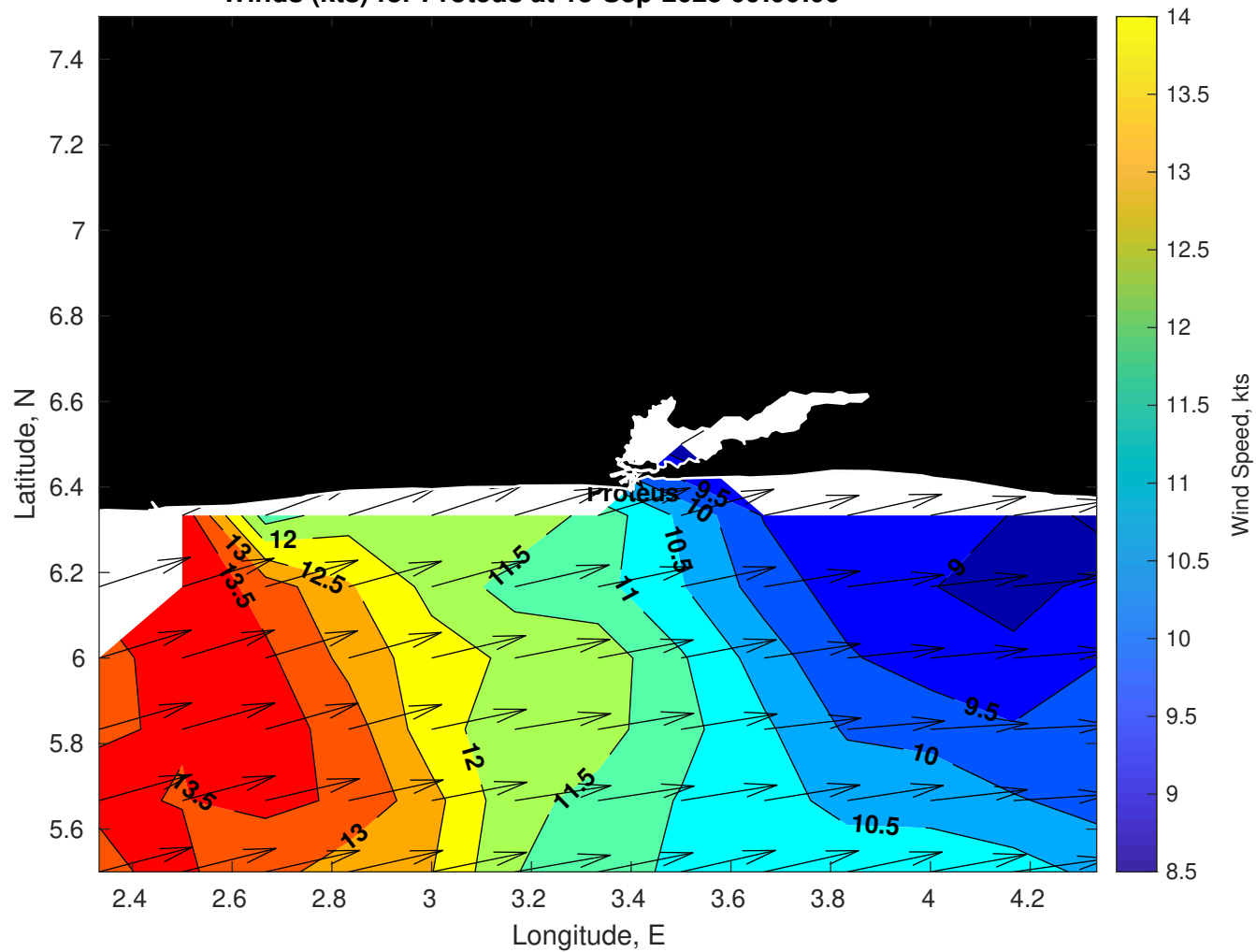
Winds (kts) for Proteus at 15-Sep-2025 09:00:00
