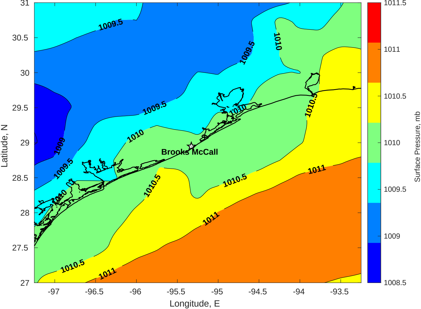
Surface Pressure (mb) for Brooks McCall at 04-Sep-2025 00:00:00
