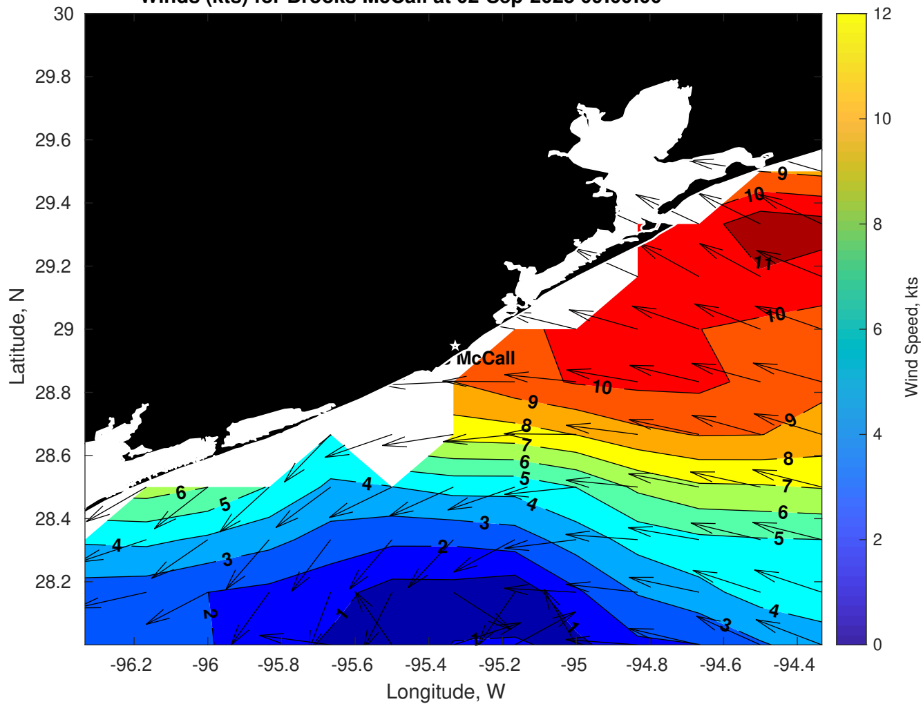
Winds (kts) for Brooks McCall at 02-Sep-2025 09:00:00
