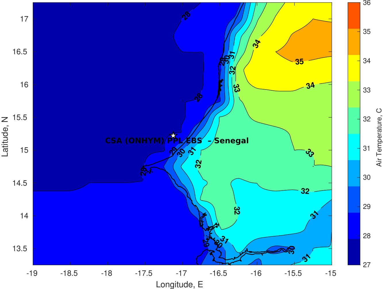
Air Temperature (C) for CSA (ONHYM) PPL EBS - Senegal at 15-Sep-2025
