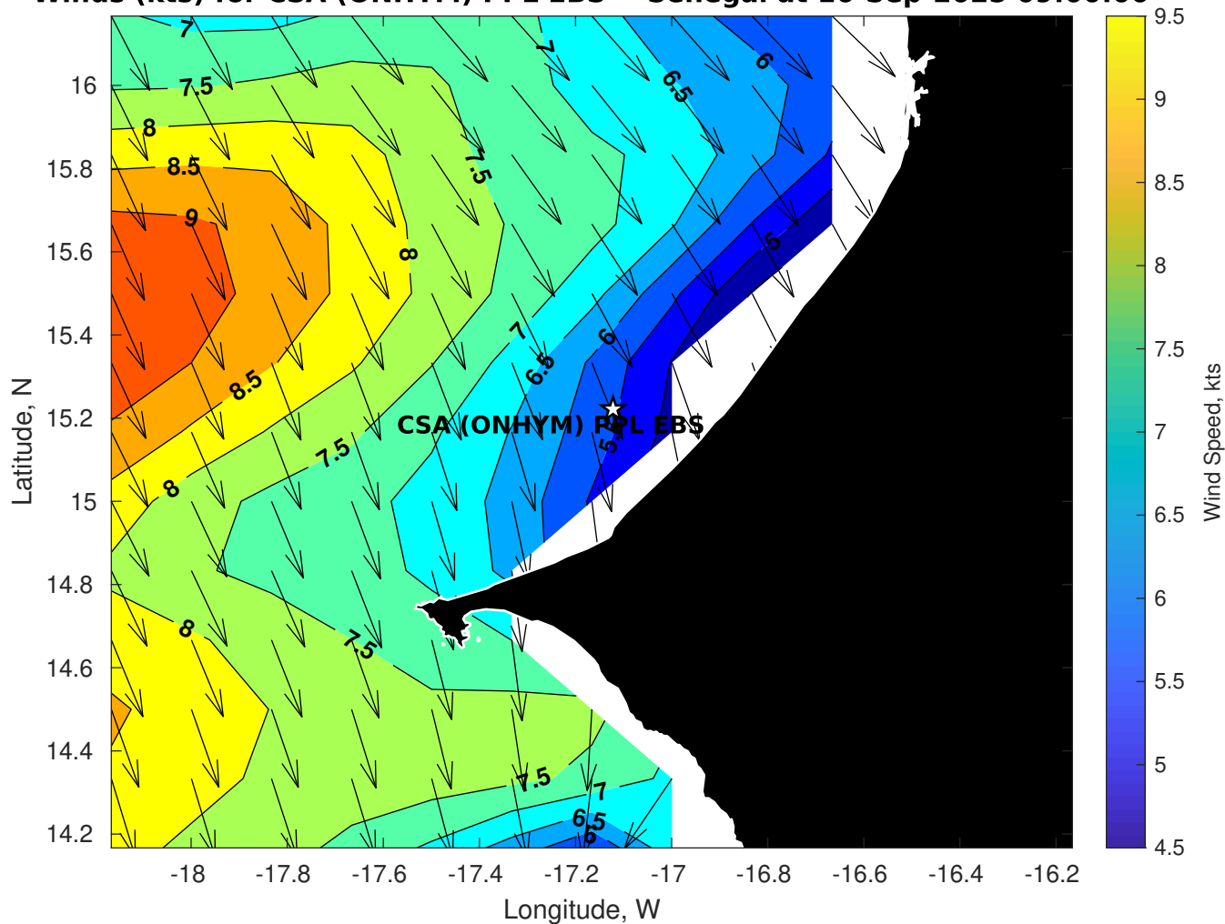
Winds (kts) for CSA (ONHYM) PPL EBS - Senegal at 16-Sep-2025 09:00:00
