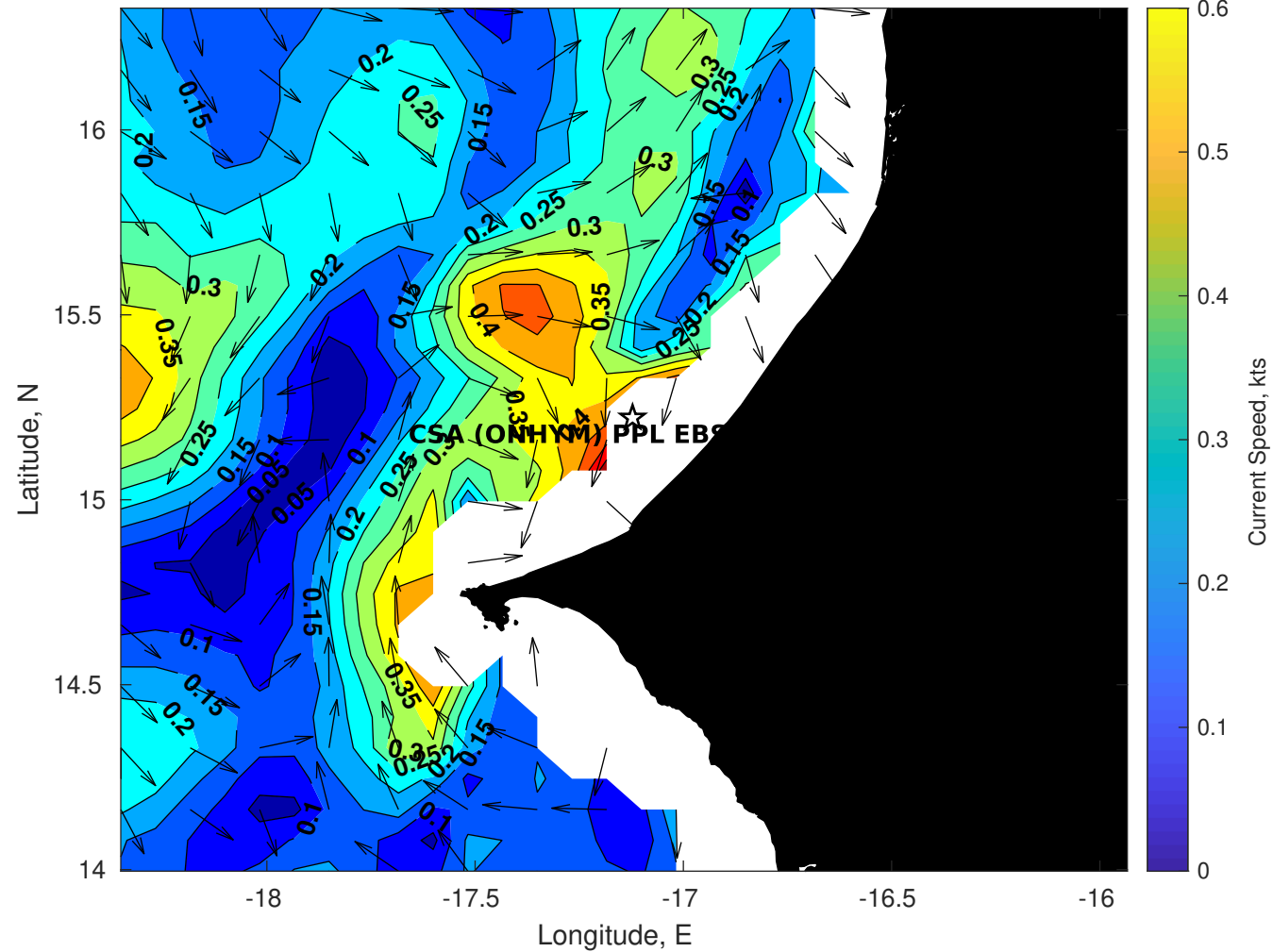
Surface Currents for CSA (ONHYM) PPL EBS - Senegal at 15-Sep-2025 00:00:00
