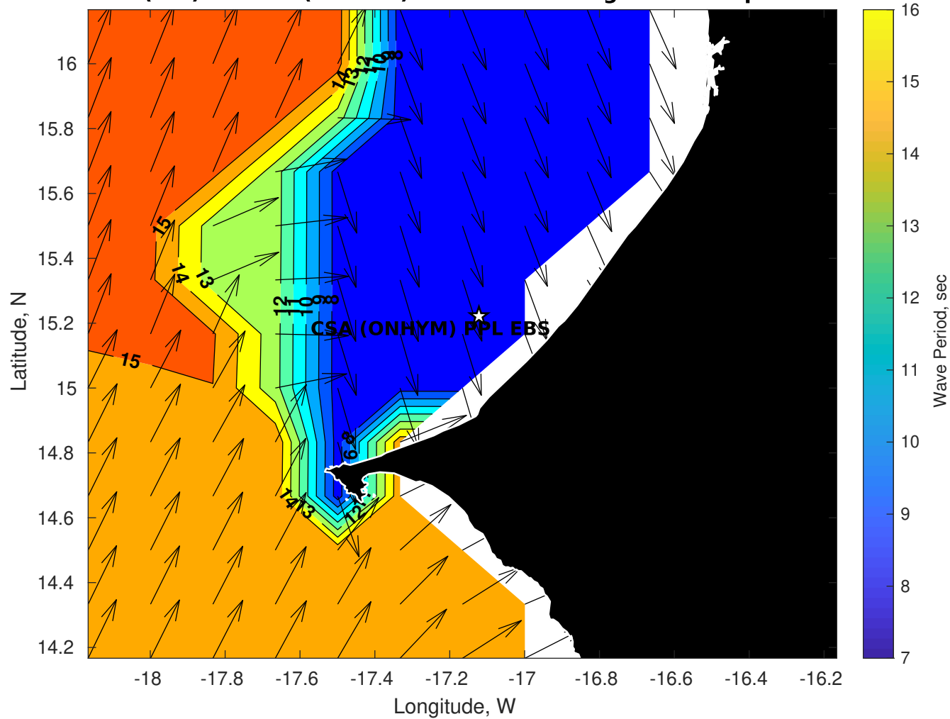
Wave Period (sec) for CSA (ONHYM) PPL EBS - Senegal at 16-Sep-2025 09:00:00
