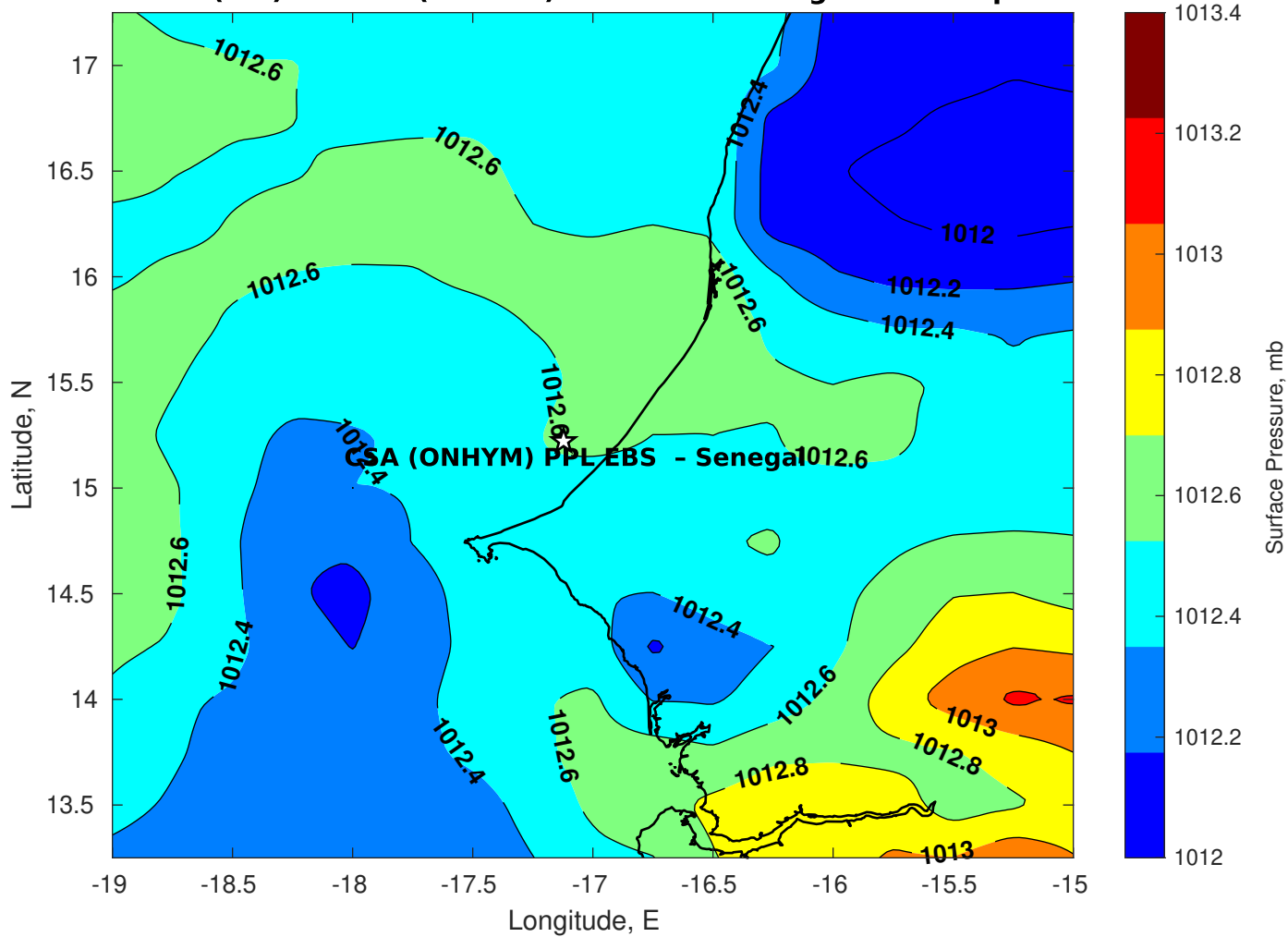
Surface Pressure (mb) for CSA (ONHYM) PPL EBS - Senegal at 16-Sep-2025 12:00:00
