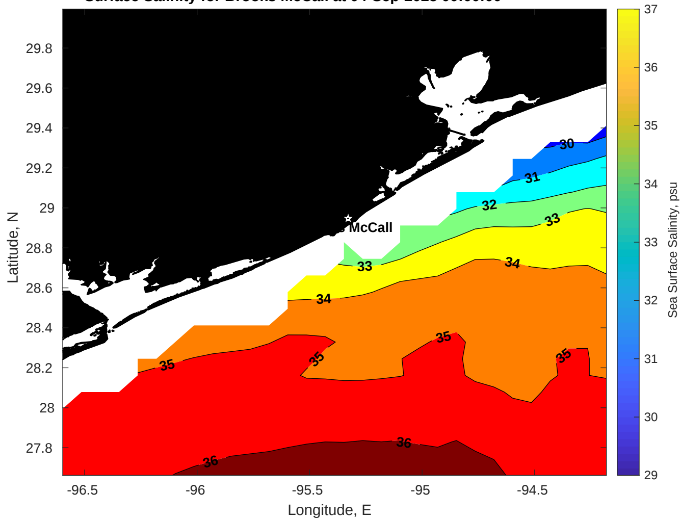
Surface Salinity for Brooks McCall at 04-Sep-2025 00:00:00
