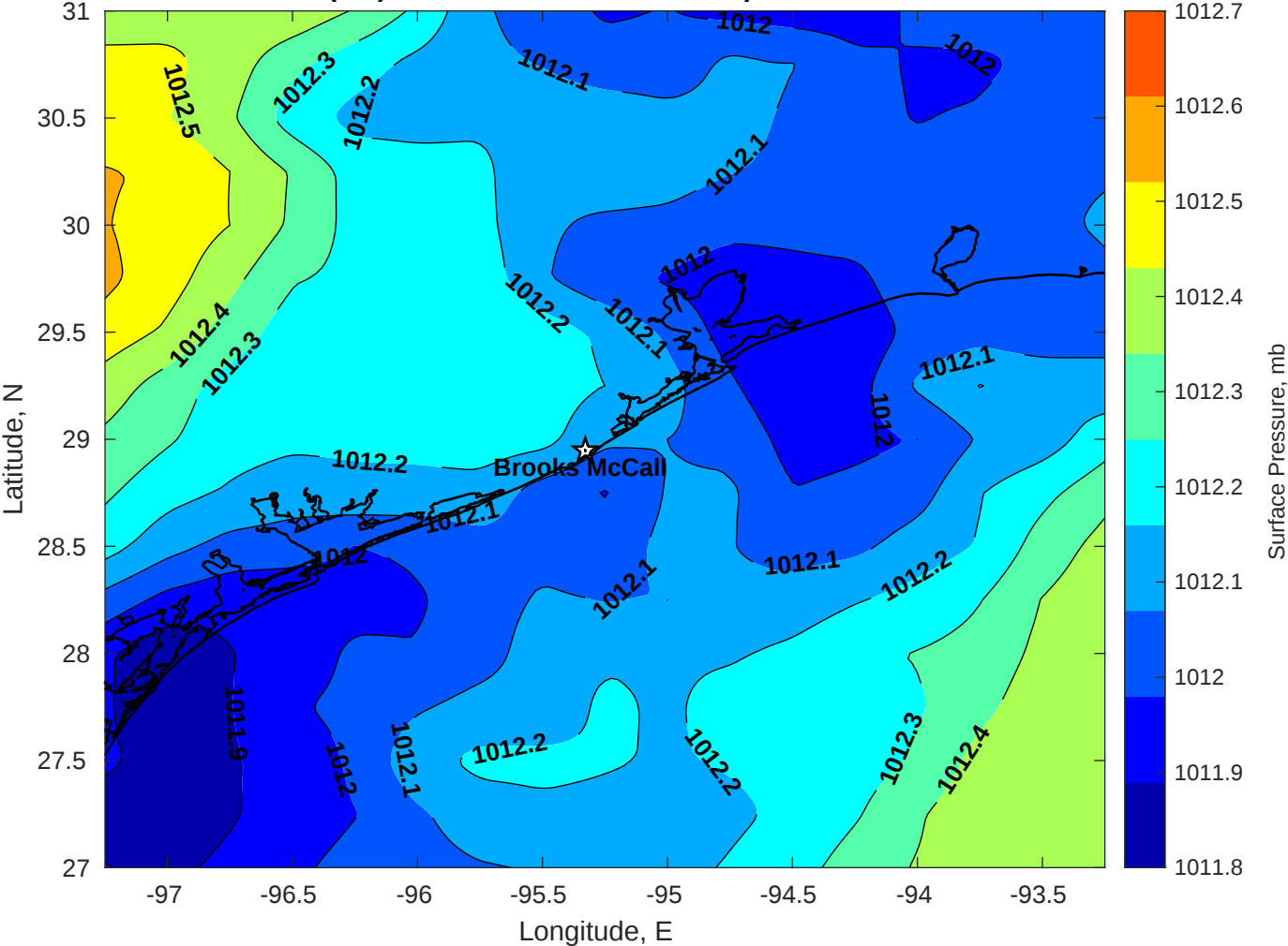
Surface Pressure (mb) for Brooks McCall at 04-Sep-2025 12:00:00
