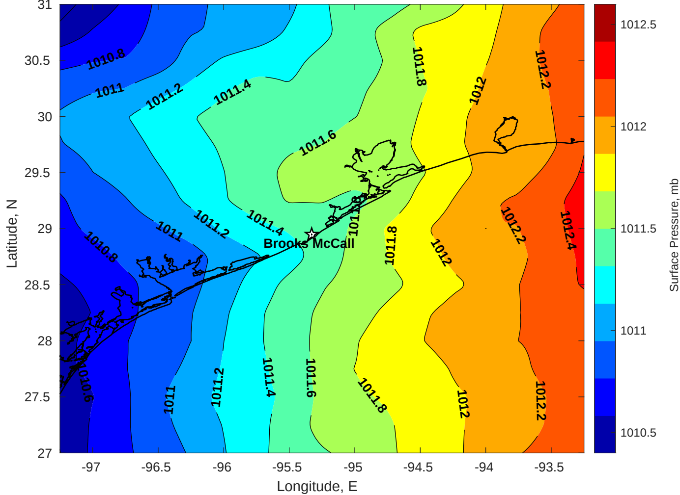
Surface Pressure (mb) for Brooks McCall at 05-Sep-2025 12:00:00
