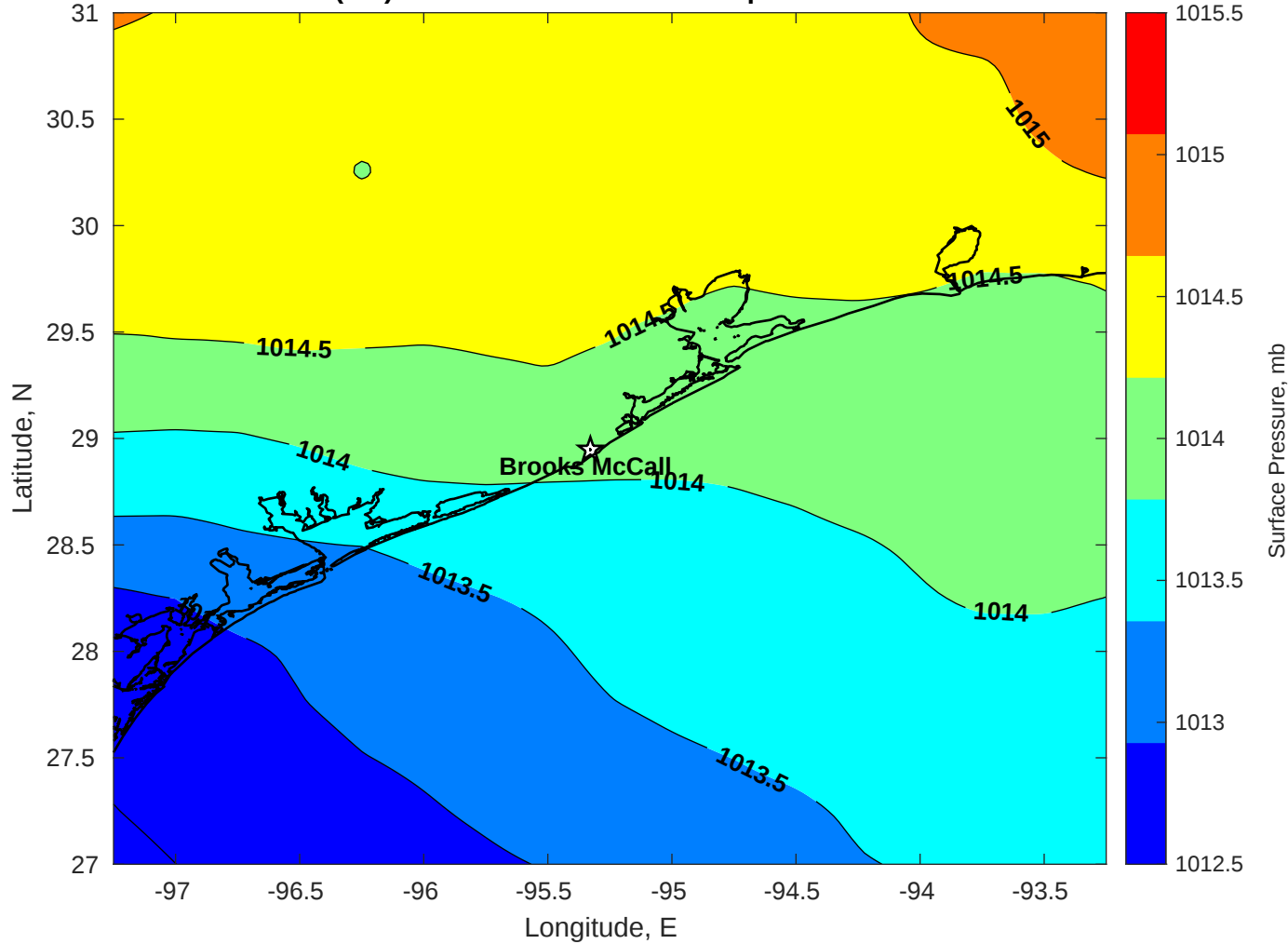
Surface Pressure (mb) for Brooks McCall at 06-Sep-2025 12:00:00
