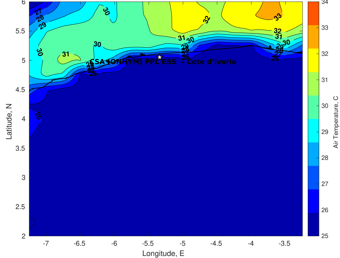
Air Temperature (C) for CSA (ONHYM) PPL EBS - Cote d'Ivoire at 04-Sep-2025
