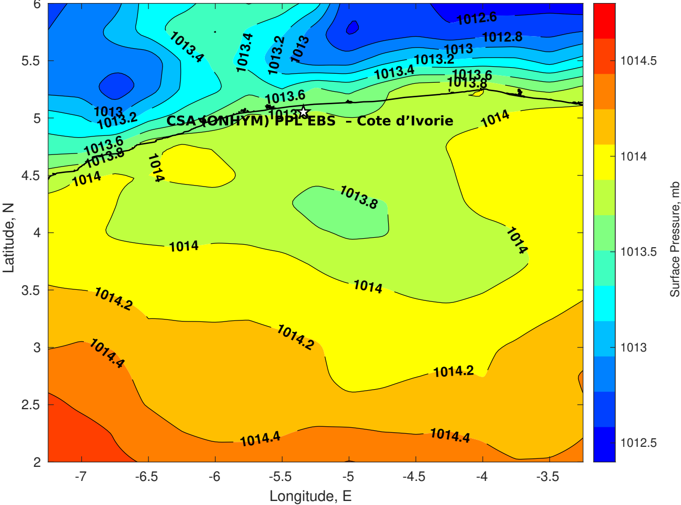
Surface Pressure (mb) for CSA (ONHYM) PPL EBS - Cote d'Ivoire at 04-Sep-2025 12:00:00
