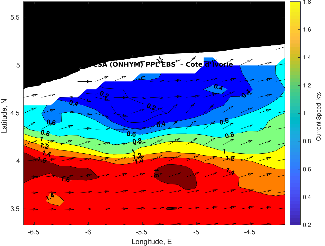
Surface Currents for CSA (ONHYM) PPL EBS - Cote d'Ivoire at 04-Sep-2025 00:00:00
