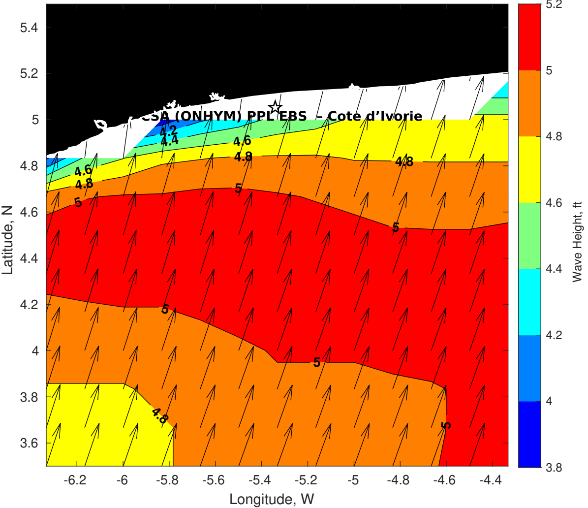
Wave Height (ft) for CSA (ONHYM) PPL EBS - Cote d'Ivoire at 04-Sep-2025 21:00:00
