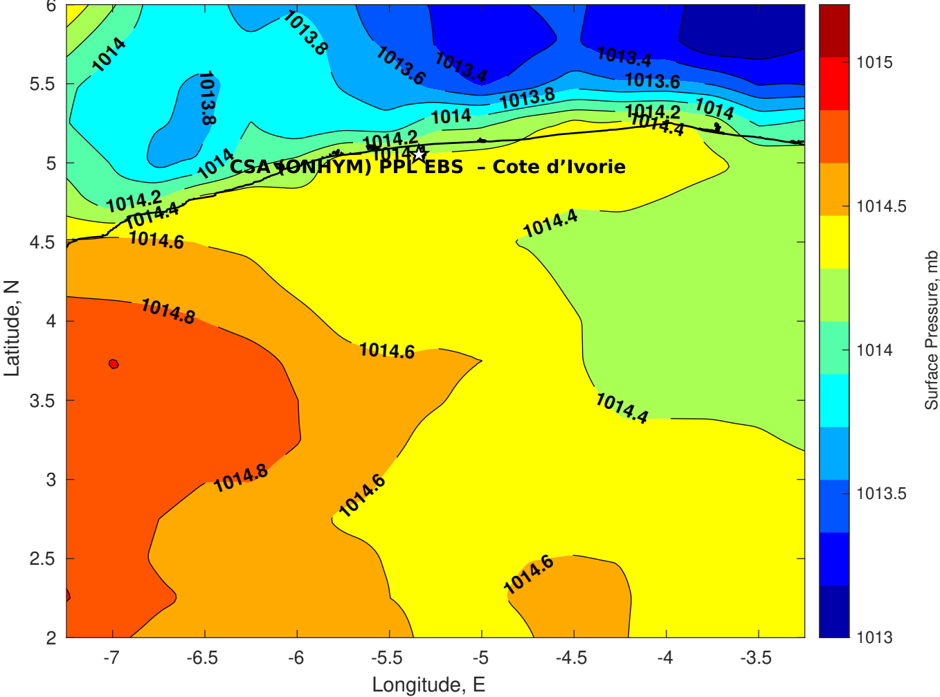
Surface Pressure (mb) for CSA (ONHYM) PPL EBS - Cote d'Ivoire at 05-Sep-2025 12:00:00
