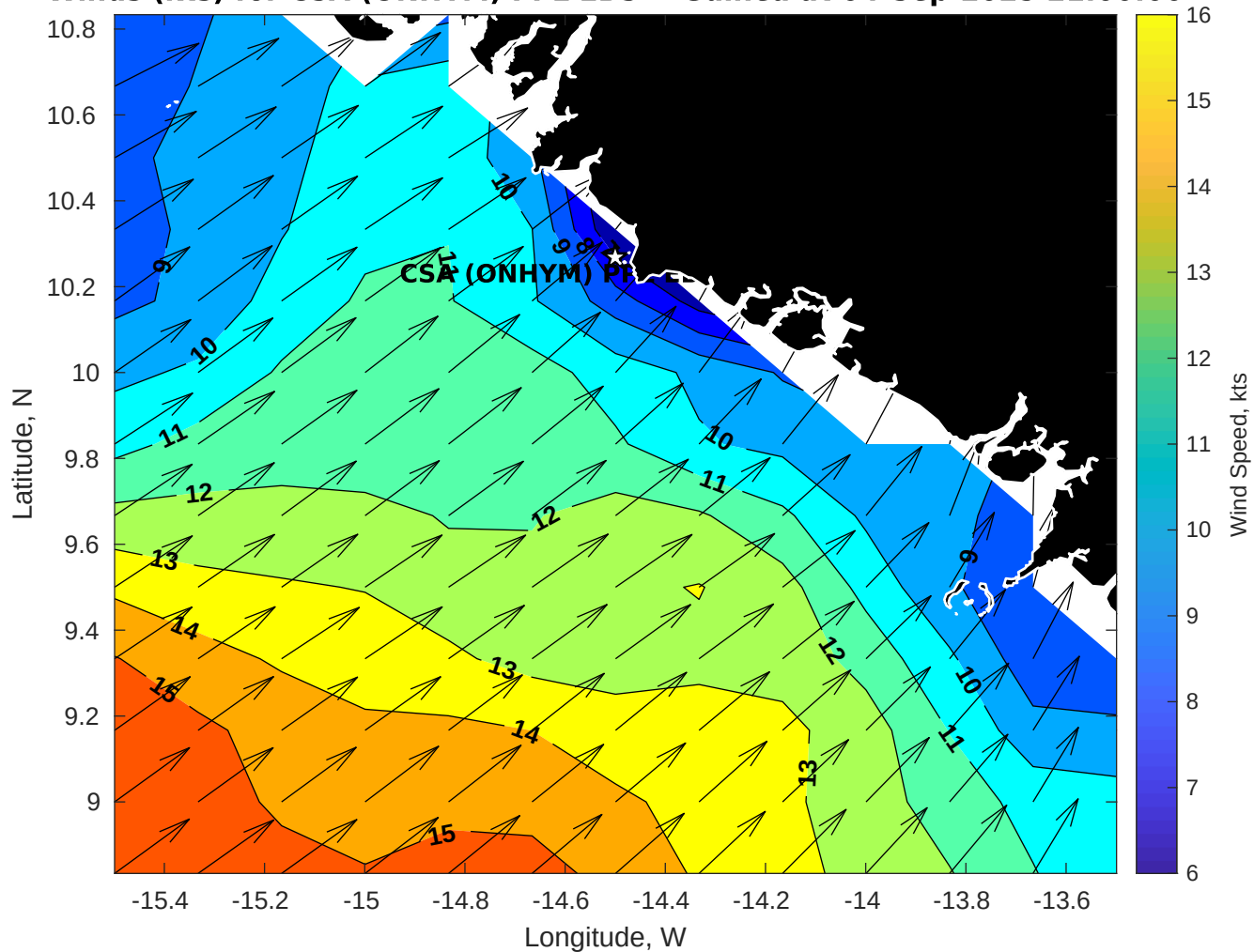
Winds (kts) for CSA (ONHYM) PPL EBS - Guinea at 04-Sep-2025 21:00:00
