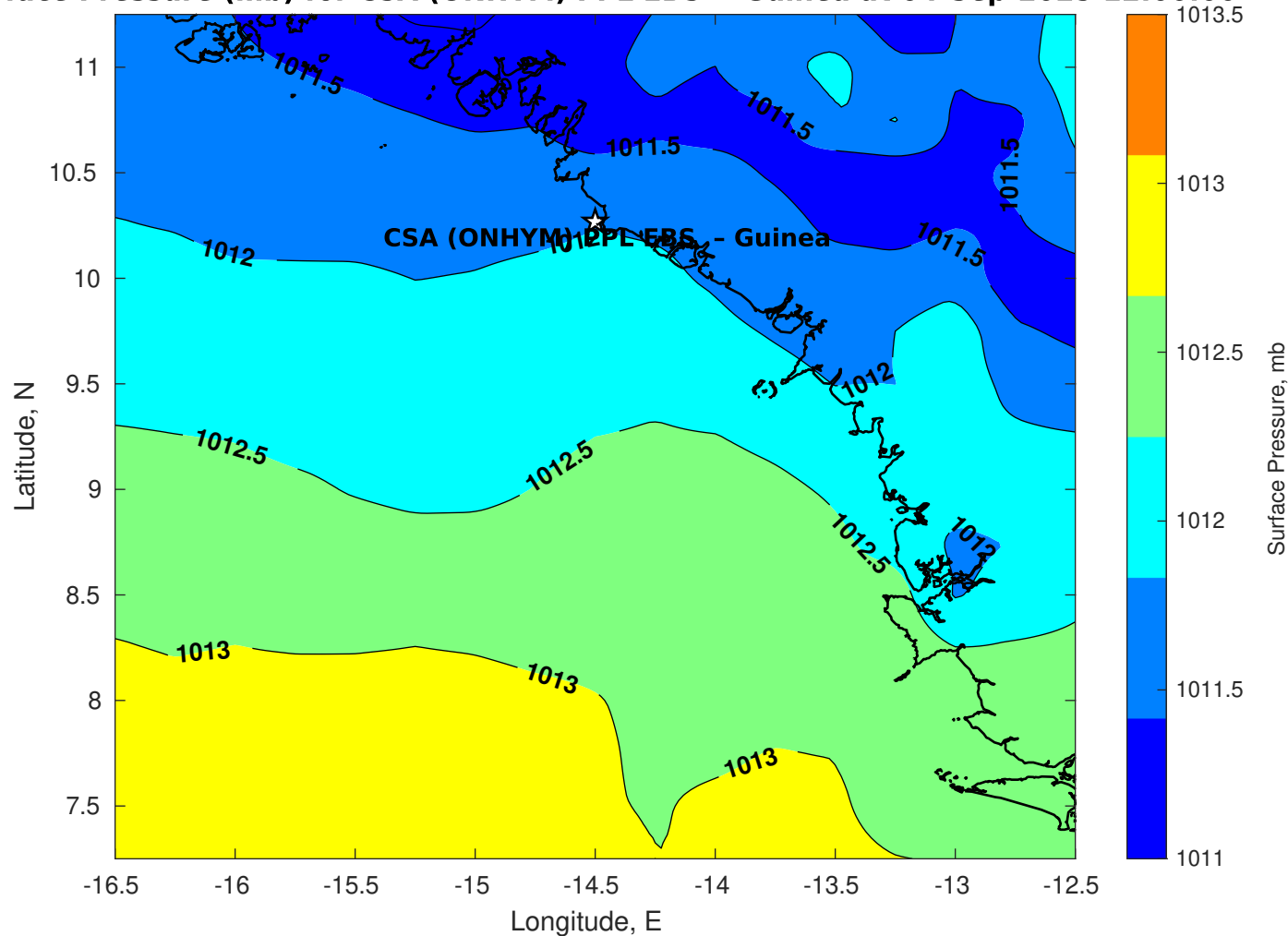
Surface Pressure (mb) for CSA (ONHYM) PPL EBS - Guinea at 04-Sep-2025 12:00:00
