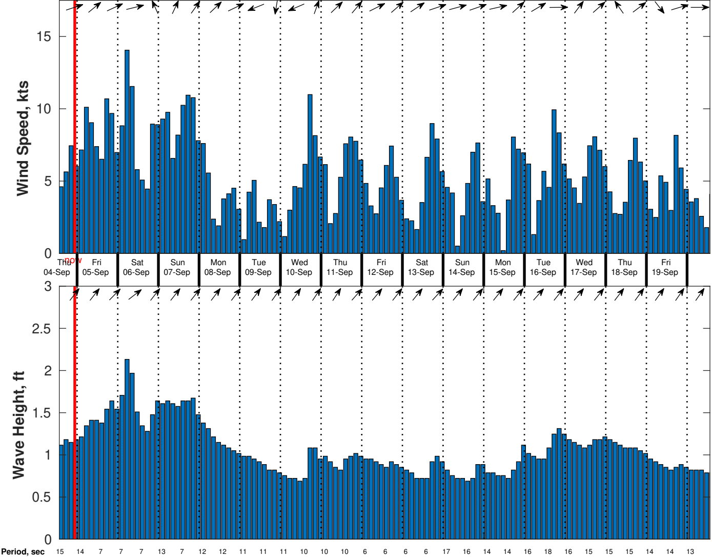
Wind & Wave Forecast for CSA (ONHYM) PPL EBS - Guinea from 04-Sep-2025 13:00:00 to 20-Sep-2025 13:00:00
