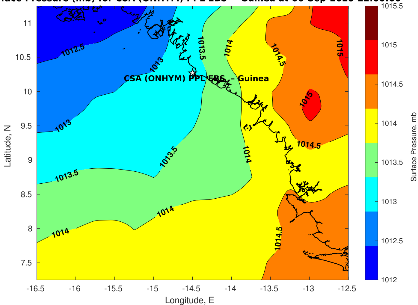
Surface Pressure (mb) for CSA (ONHYM) PPL EBS - Guinea at 06-Sep-2025 12:00:00
