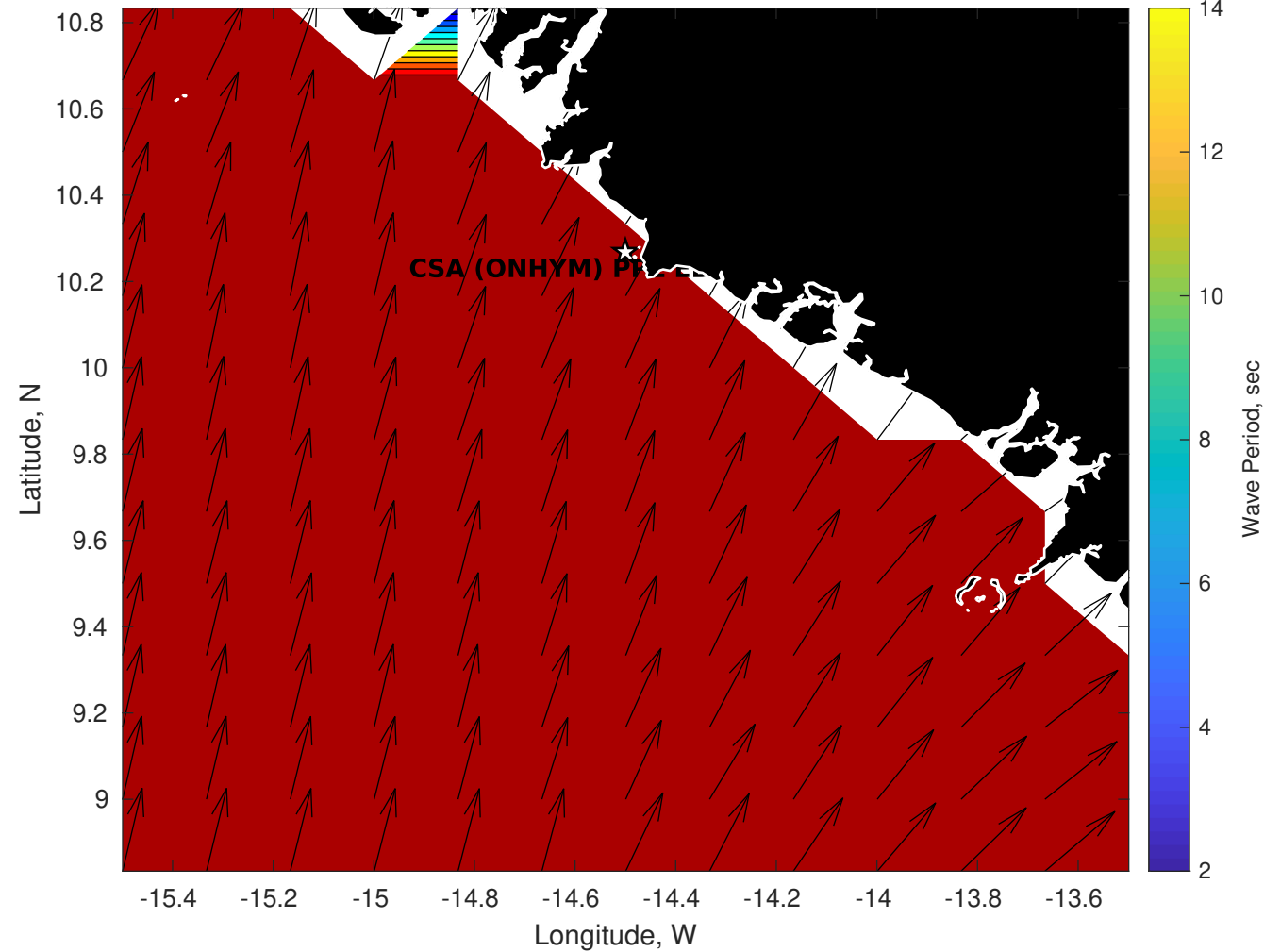
Wave Period (sec) for CSA (ONHYM) PPL EBS - Guinea at 04-Sep-2025 21:00:00
