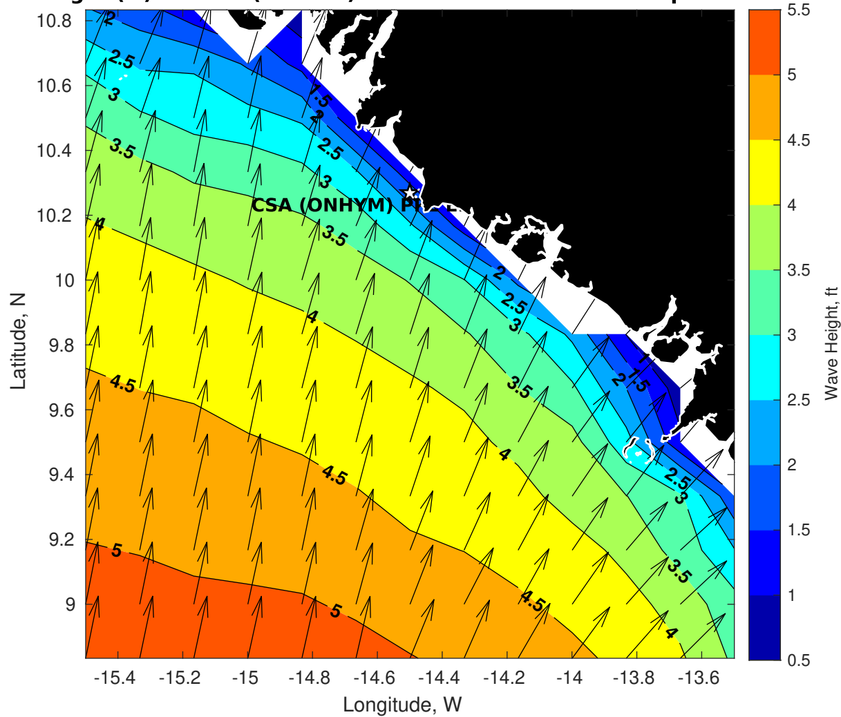
Wave Height (ft) for CSA (ONHYM) PPL EBS - Guinea at 04-Sep-2025 21:00:00
