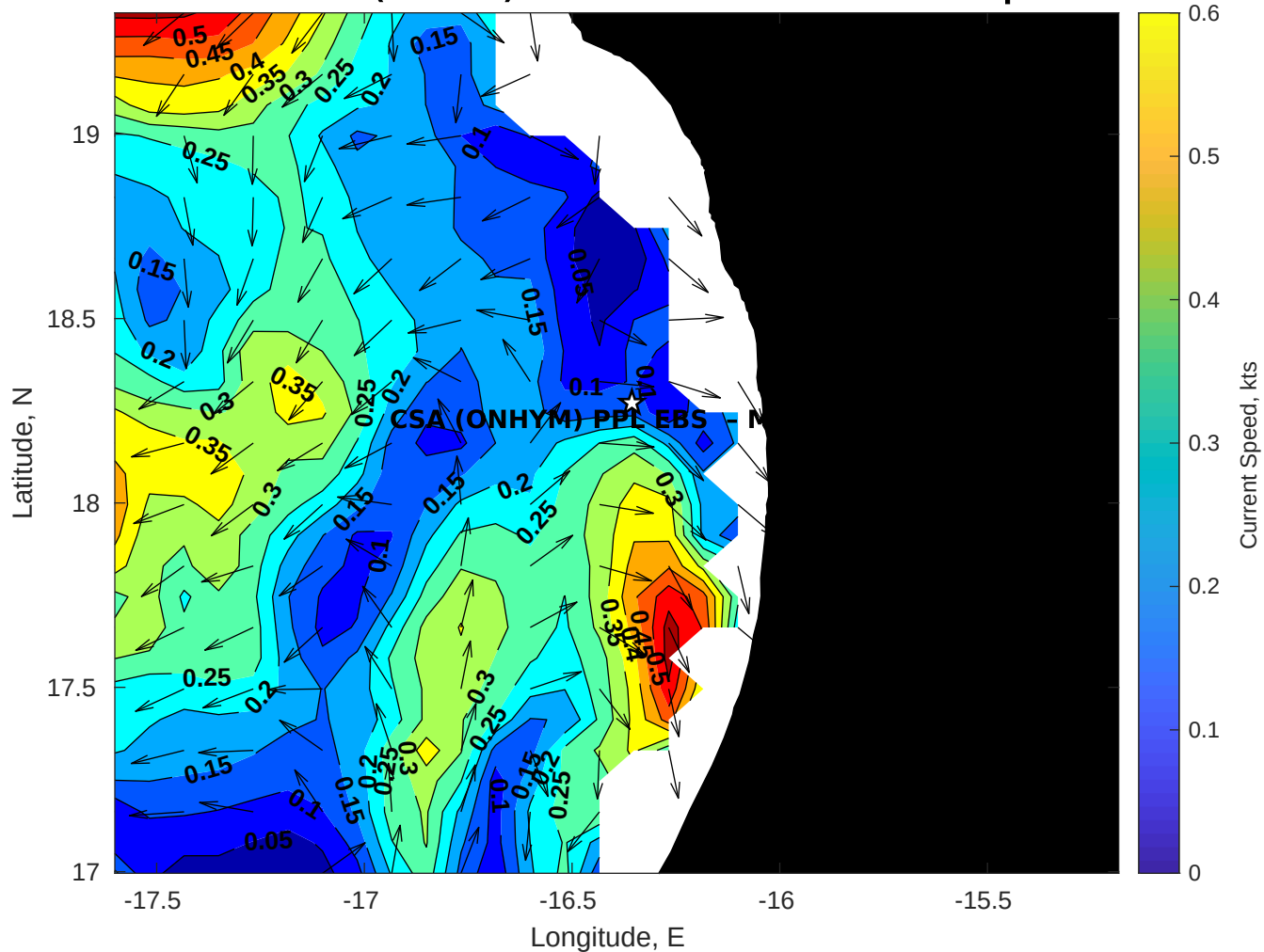
Surface Currents for CSA (ONHYM) PPL EBS - Mauritania at 04-Sep-2025 00:00:00
