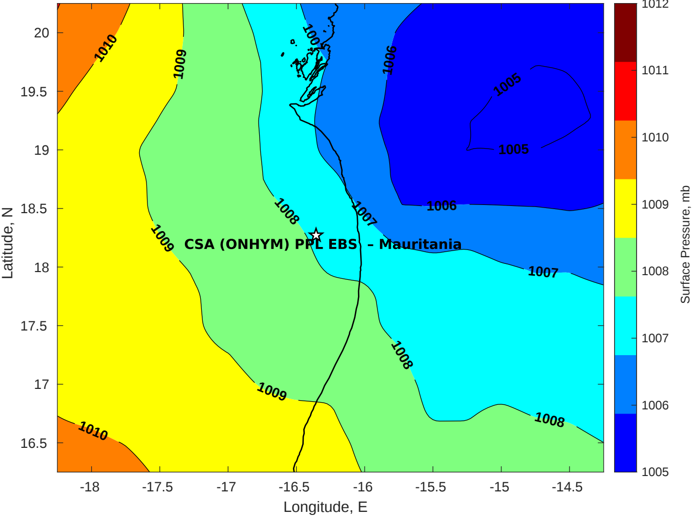
Surface Pressure (mb) for CSA (ONHYM) PPL EBS - Mauritania at 05-Sep-2025 12:00:00
