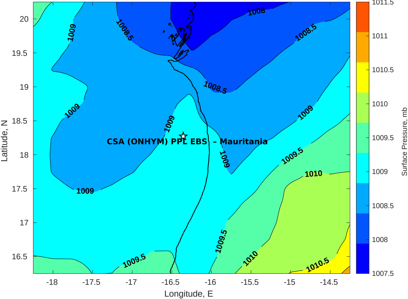
Surface Pressure (mb) for CSA (ONHYM) PPL EBS - Mauritania at 06-Sep-2025 12:00:00
