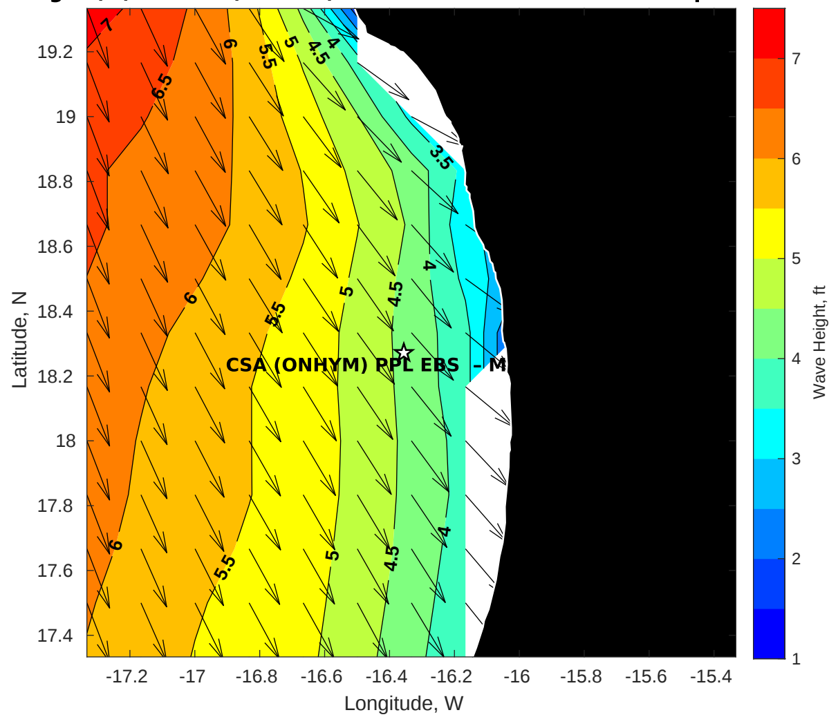
Wave Height (ft) for CSA (ONHYM) PPL EBS - Mauritania at 04-Sep-2025 21:00:00
