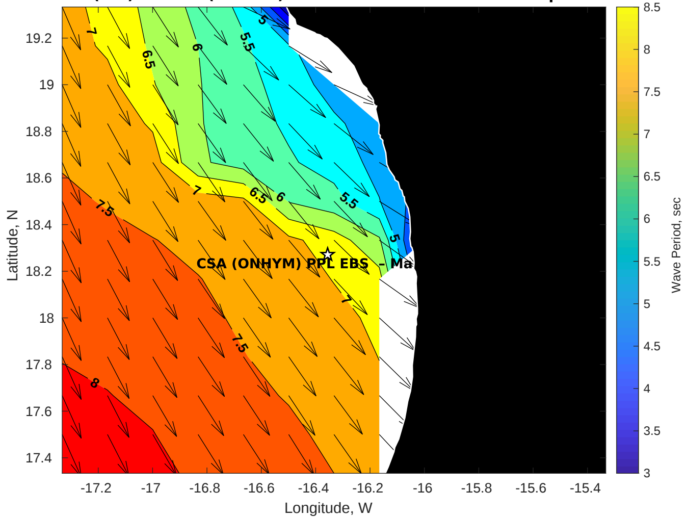
Wave Period (sec) for CSA (ONHYM) PPL EBS - Mauritania at 04-Sep-2025 21:00:00
