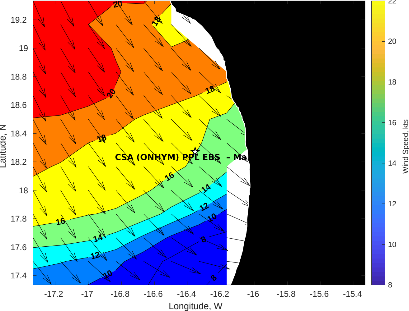
Winds (kts) for CSA (ONHYM) PPL EBS - Mauritania at 04-Sep-2025 21:00:00
