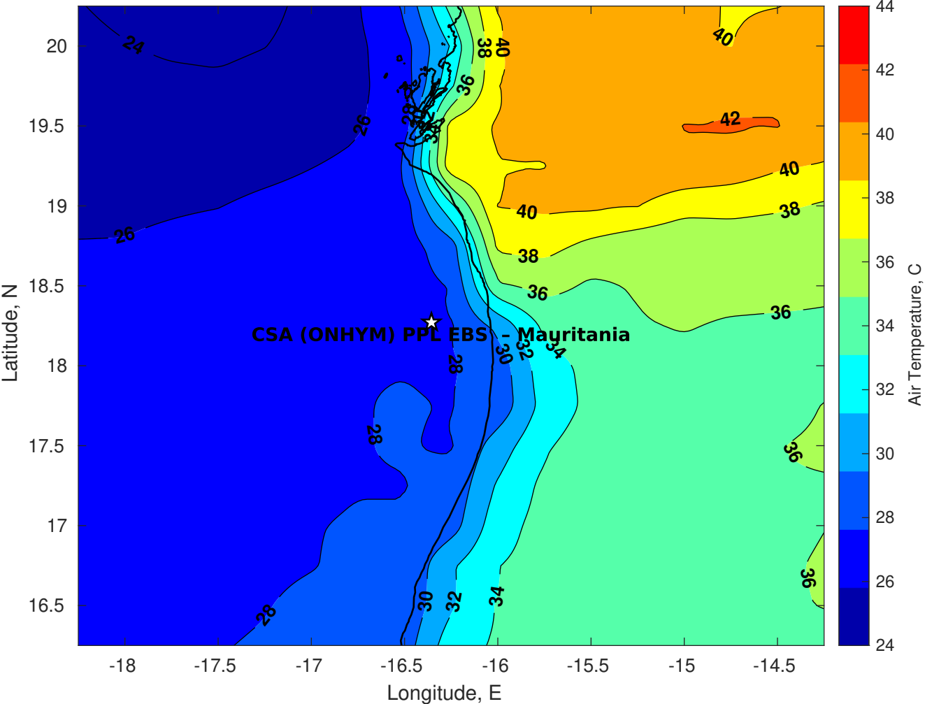
Air Temperature (C) for CSA (ONHYM) PPL EBS - Mauritania at 04-Sep-2025
