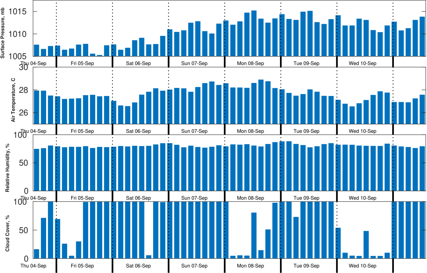
Met Forecast for CSA (ONHYM) PPL EBS - Mauritania from 04-Sep-2025 12:00:00 to 11-Sep-2025 12:00:00
