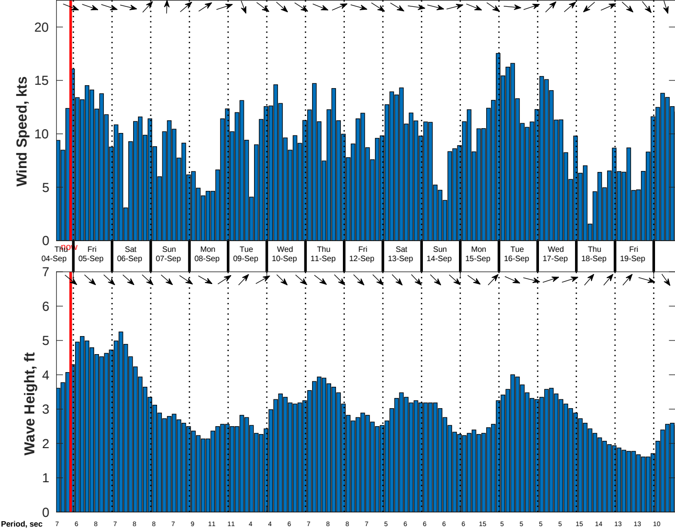
Wind & Wave Forecast for CSA (ONHYM) PPL EBS - Mauritania from 04-Sep-2025 13:00:00 to 20-Sep-2025 13:00:00
