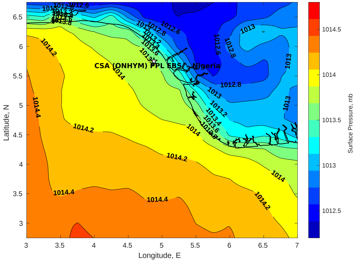
Surface Pressure (mb) for CSA (ONHYM) PPL EBS - Nigeria at 06-Sep-2025 12:00:00
