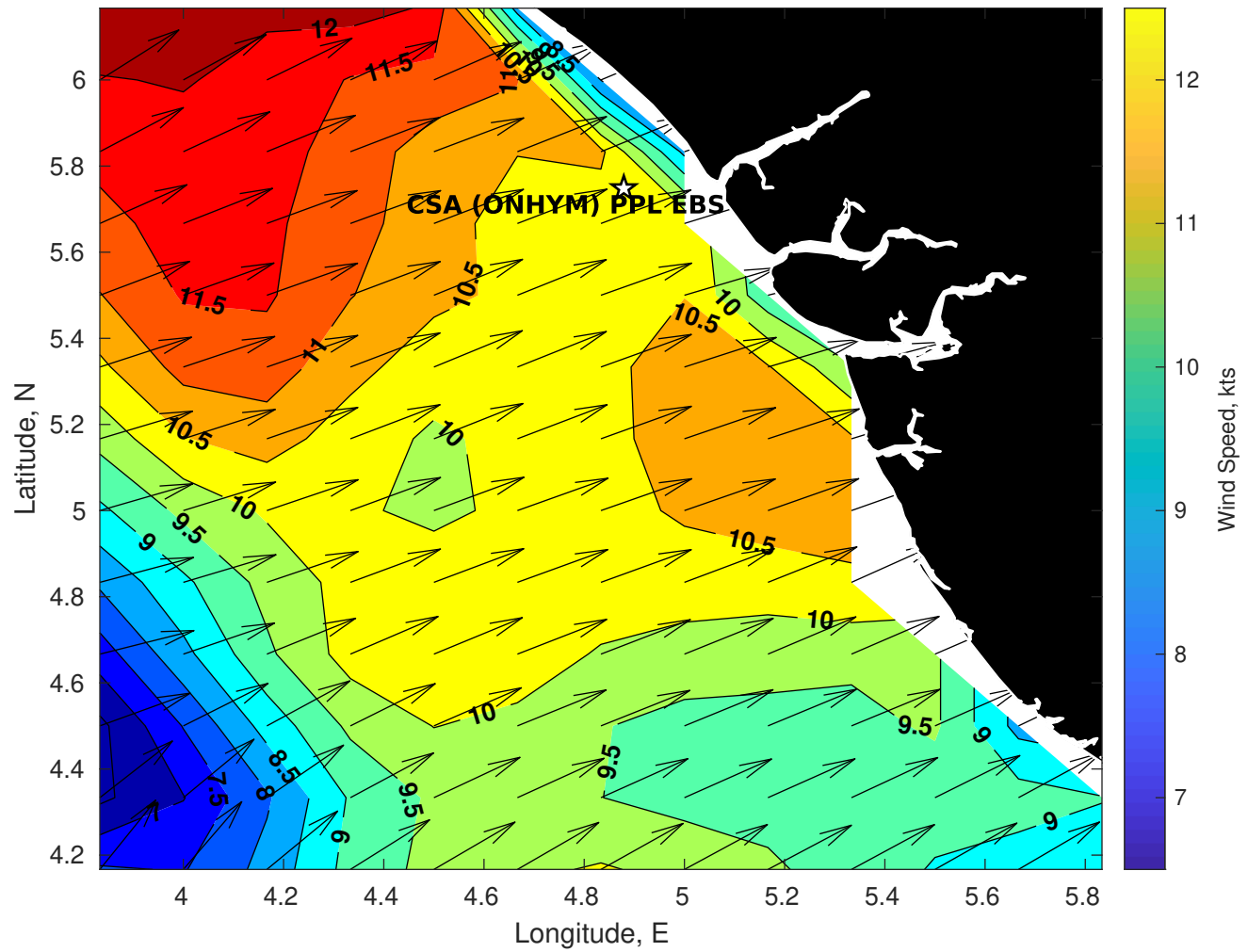
Winds (kts) for CSA (ONHYM) PPL EBS - Nigeria at 04-Sep-2025 21:00:00
