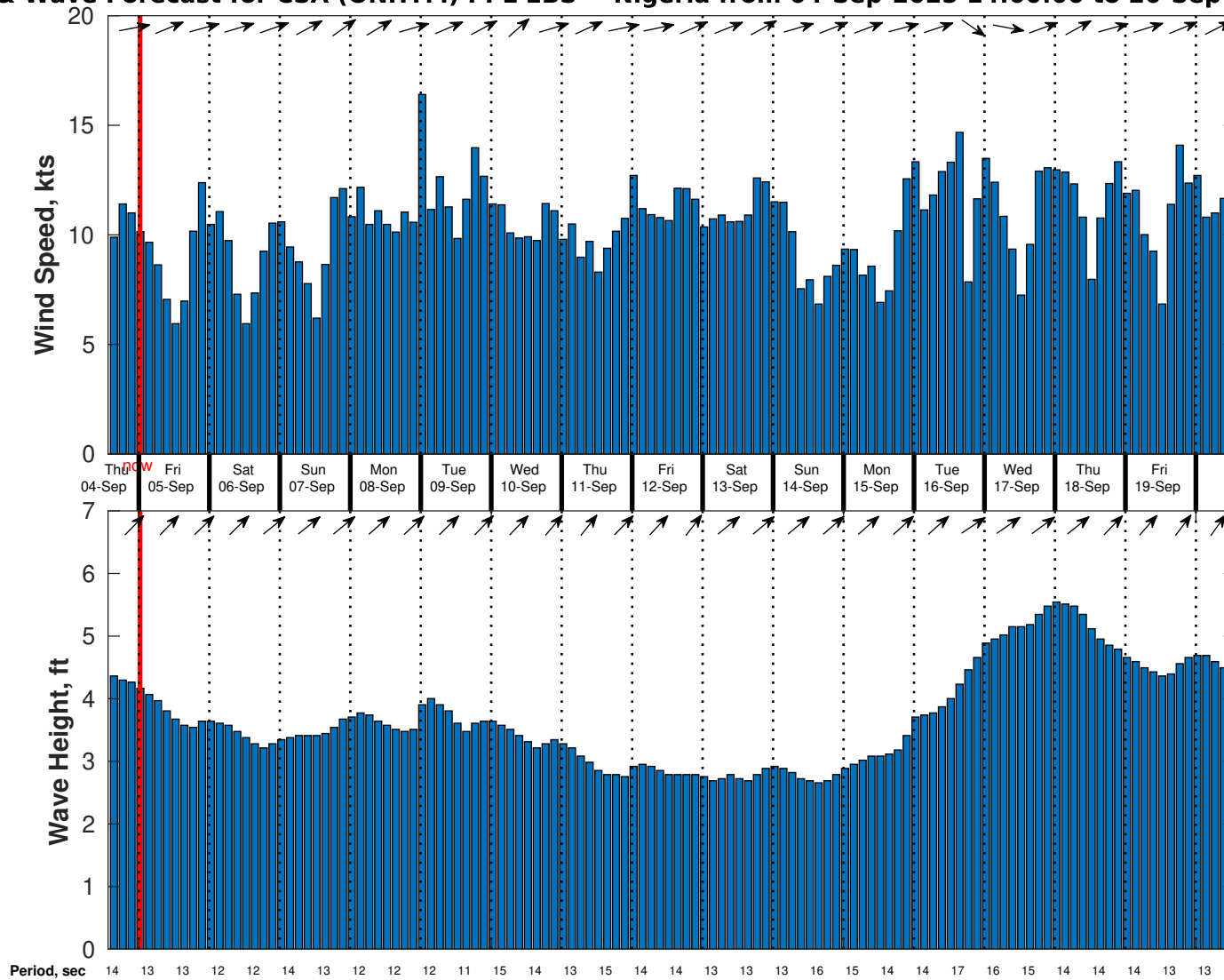
Wind & Wave Forecast for CSA (ONHYM) PPL EBS - Nigeria from 04-Sep-2025 14:00:00 to 20-Sep-2025 14:00:00
