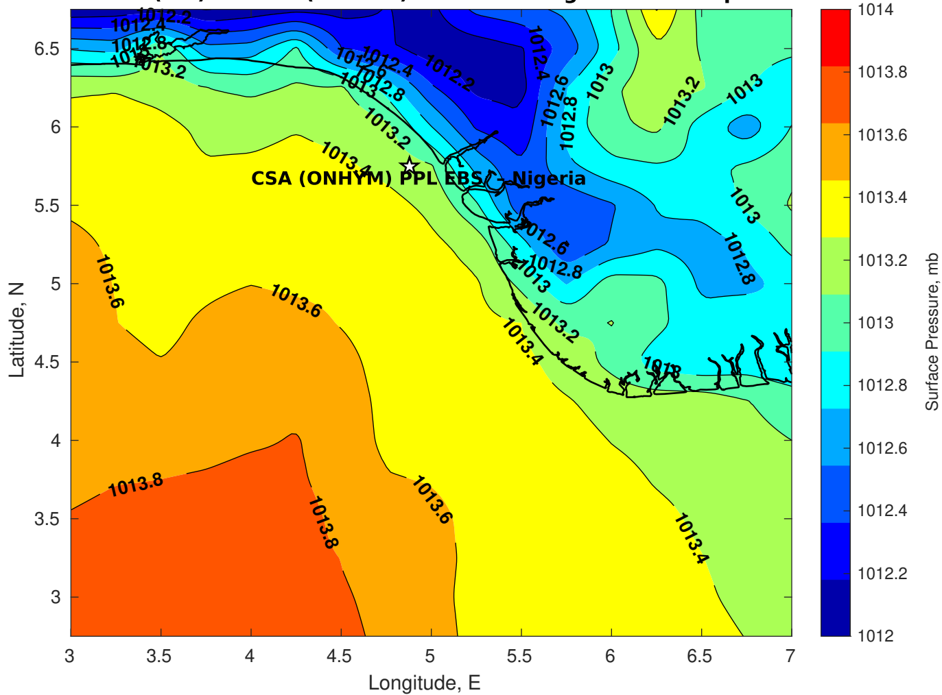
Surface Pressure (mb) for CSA (ONHYM) PPL EBS - Nigeria at 05-Sep-2025 12:00:00
