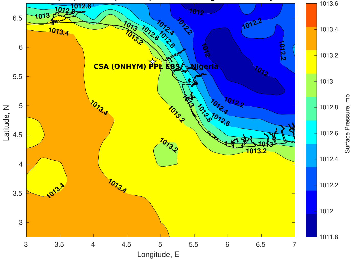
Surface Pressure (mb) for CSA (ONHYM) PPL EBS - Nigeria at 04-Sep-2025 12:00:00
