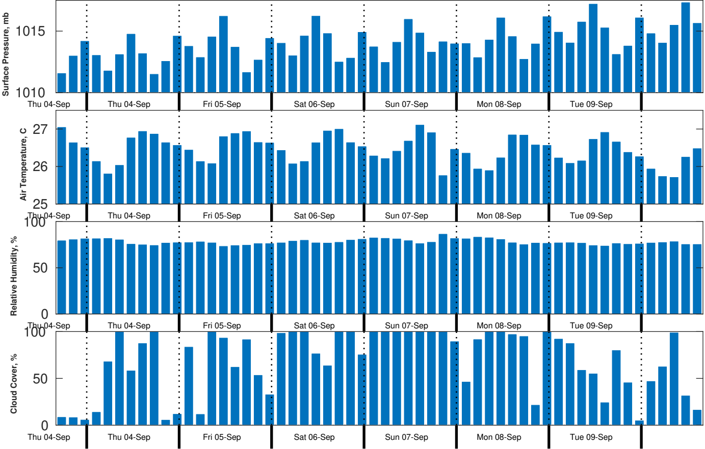
Met Forecast for CSA (ONHYM) PPL EBS - Nigeria from 04-Sep-2025 12:00:00 to 11-Sep-2025 12:00:00
