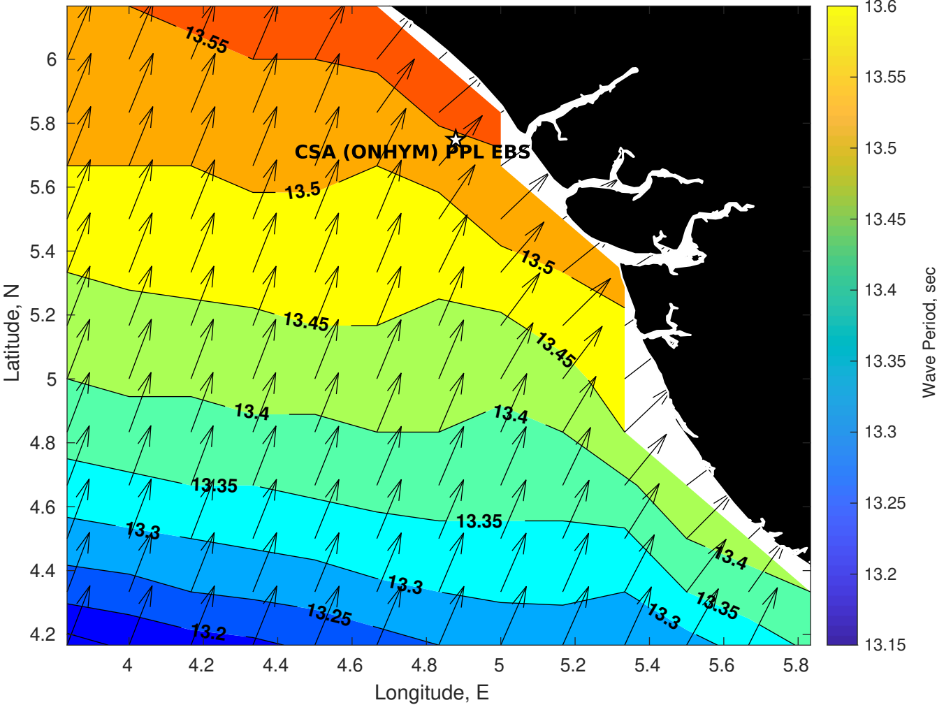
Wave Period (sec) for CSA (ONHYM) PPL EBS - Nigeria at 04-Sep-2025 21:00:00
