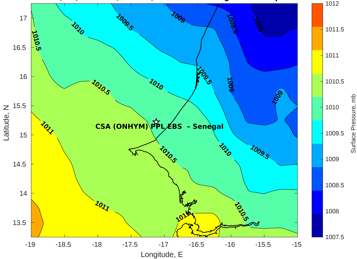
Surface Pressure (mb) for CSA (ONHYM) PPL EBS - Senegal at 05-Sep-2025 12:00:00
