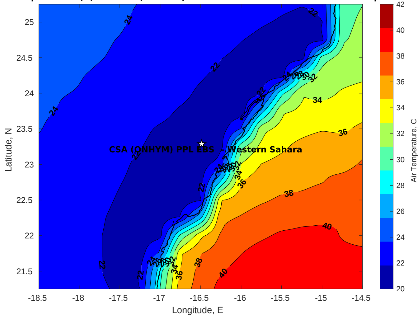
Air Temperature (C) for CSA (ONHYM) PPL EBS - Western Sahara at 04-Sep-2025
