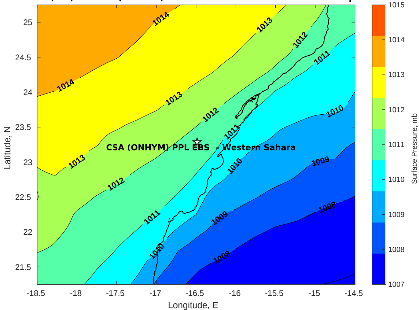
Surface Pressure (mb) for CSA (ONHYM) PPL EBS - Western Sahara at 05-Sep-2025 12:00:00
