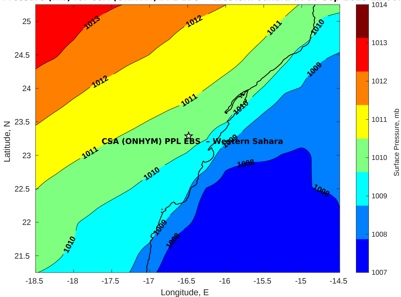
Surface Pressure (mb) for CSA (ONHYM) PPL EBS - Western Sahara at 06-Sep-2025 12:00:00
