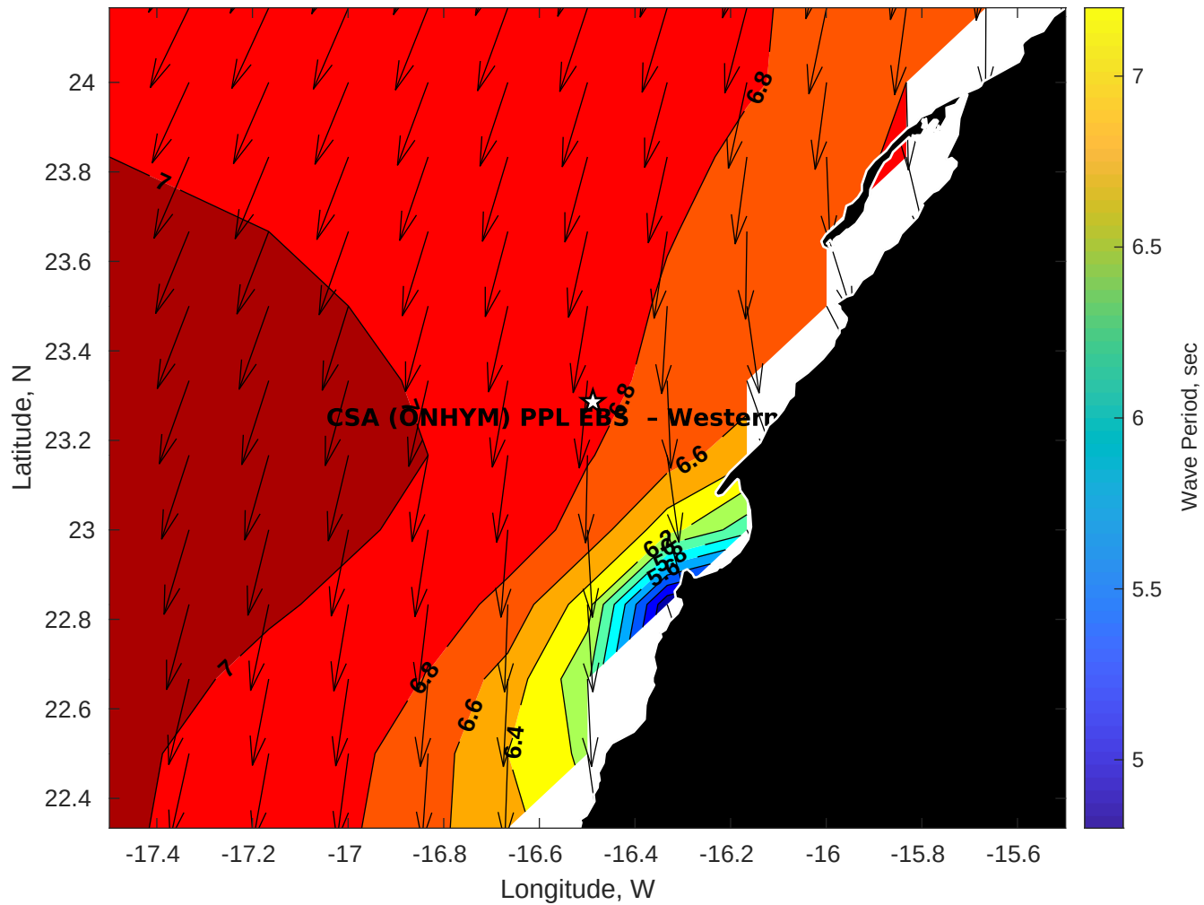
Wave Period (sec) for CSA (ONHYM) PPL EBS - Western Sahara at 04-Sep-2025 21:00:00
