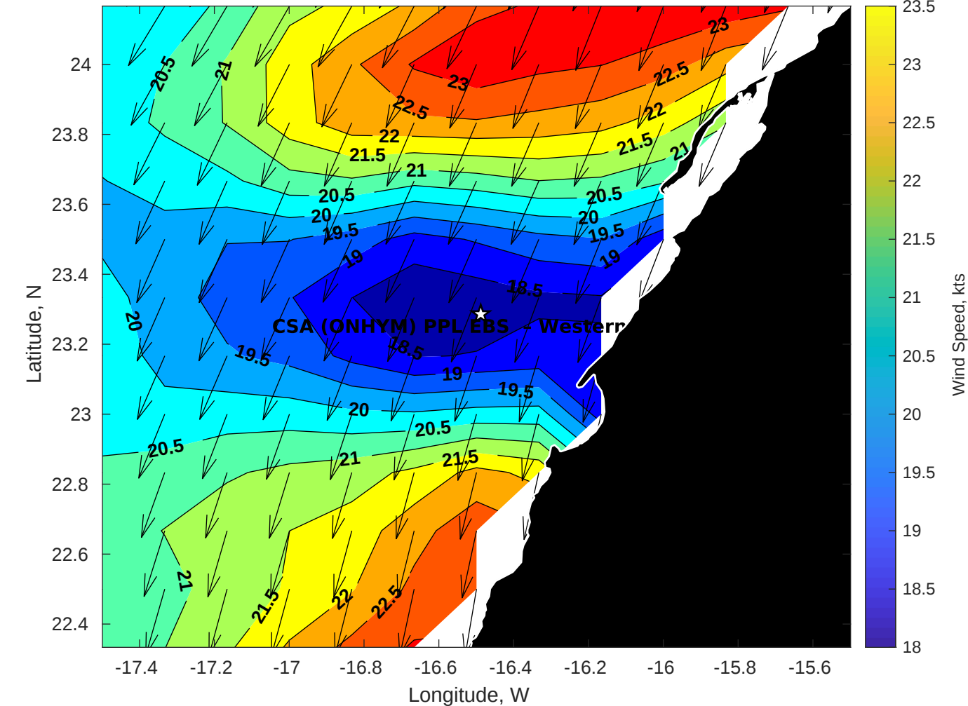
Winds (kts) for CSA (ONHYM) PPL EBS - Western Sahara at 04-Sep-2025 21:00:00
