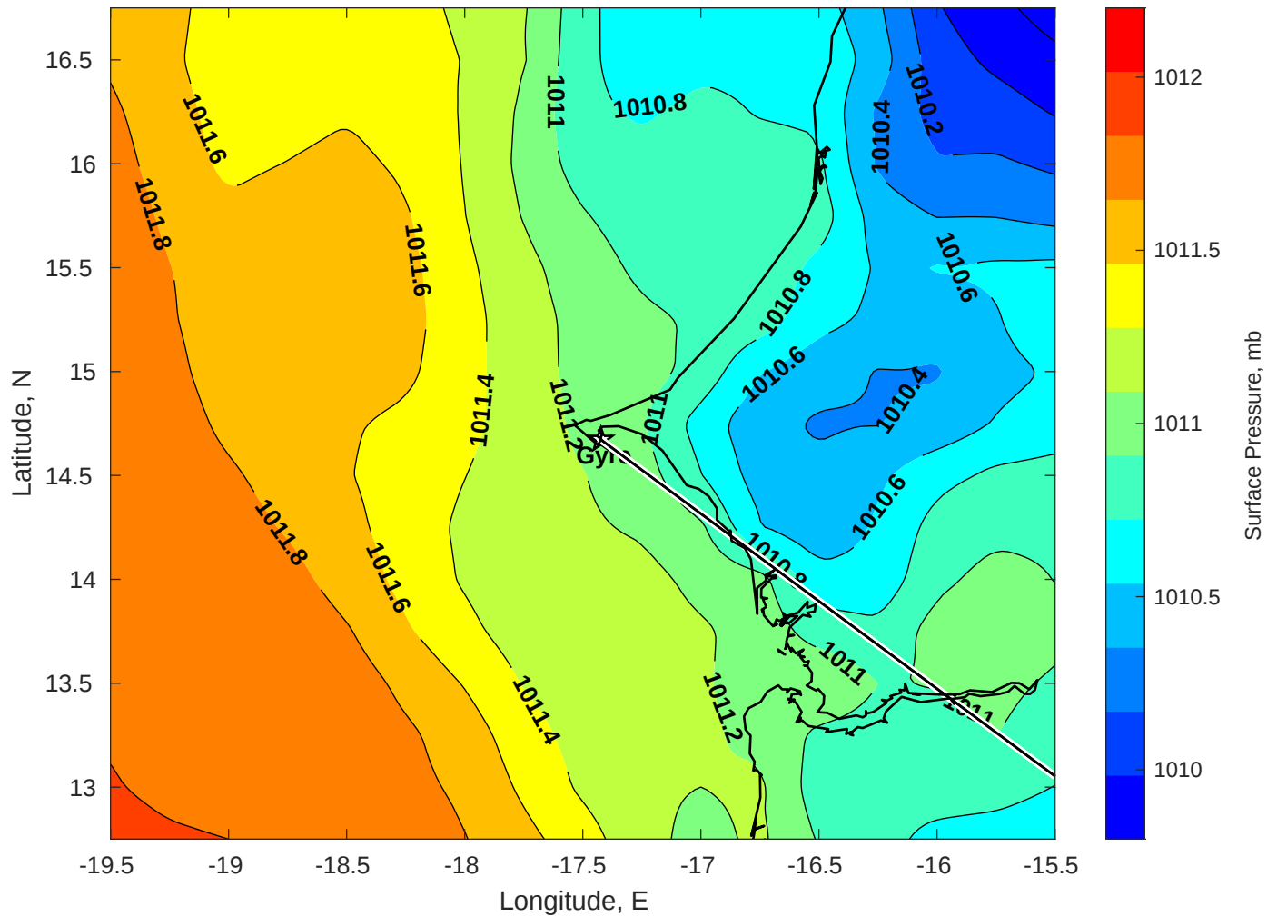
Surface Pressure (mb) for Gyre at 04-Sep-2025 12:00:00
