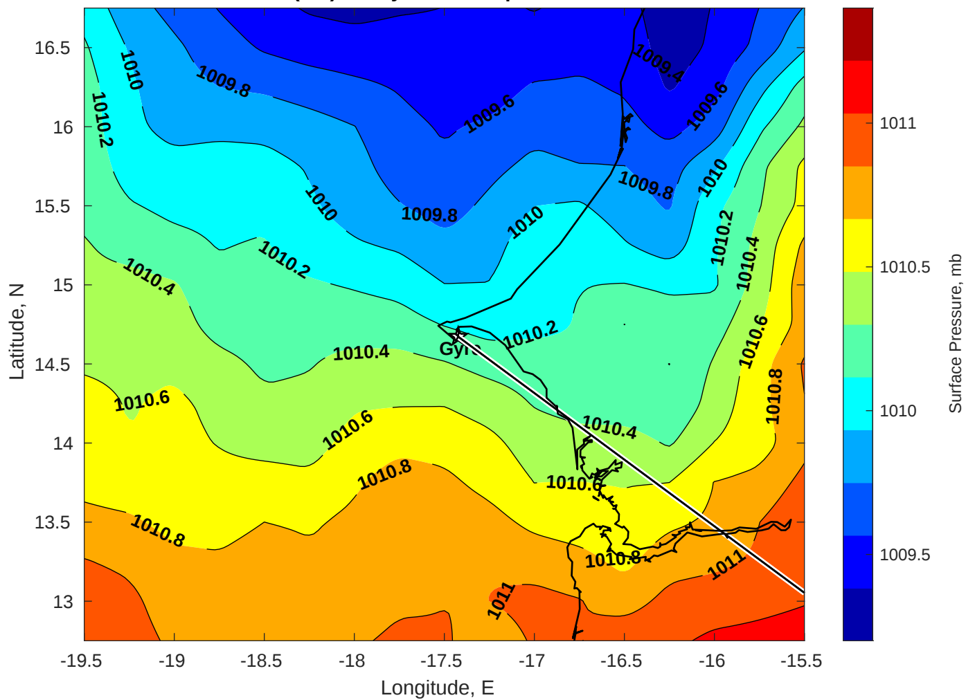
Surface Pressure (mb) for Gyre at 06-Sep-2025 12:00:00
