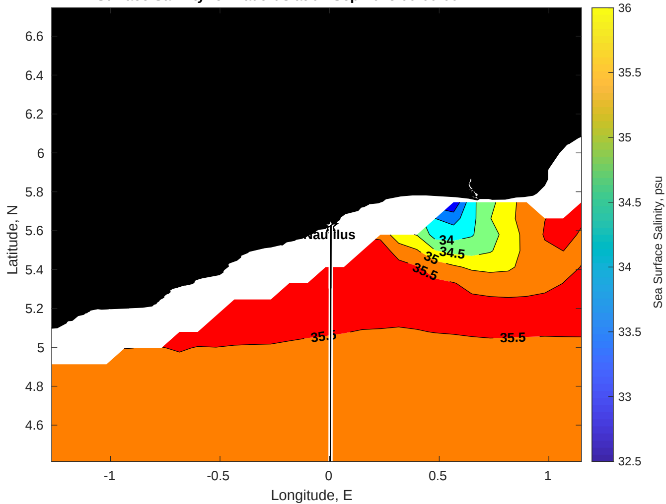
Surface Salinity for Nautilus at 04-Sep-2025 00:00:00
