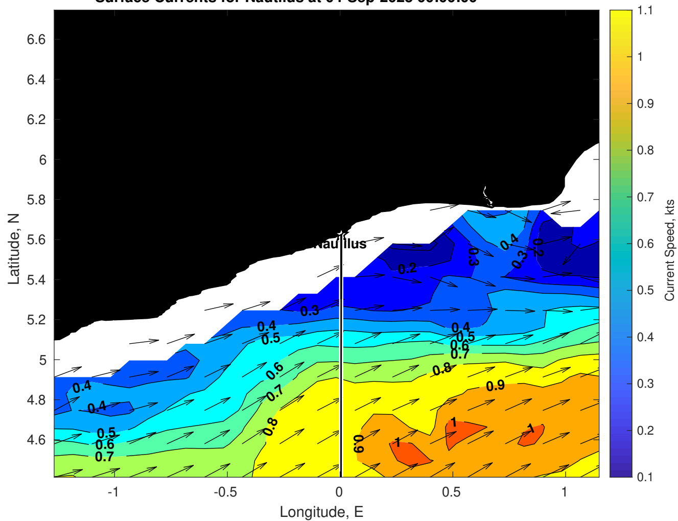
Surface Currents for Nautilus at 04-Sep-2025 00:00:00
