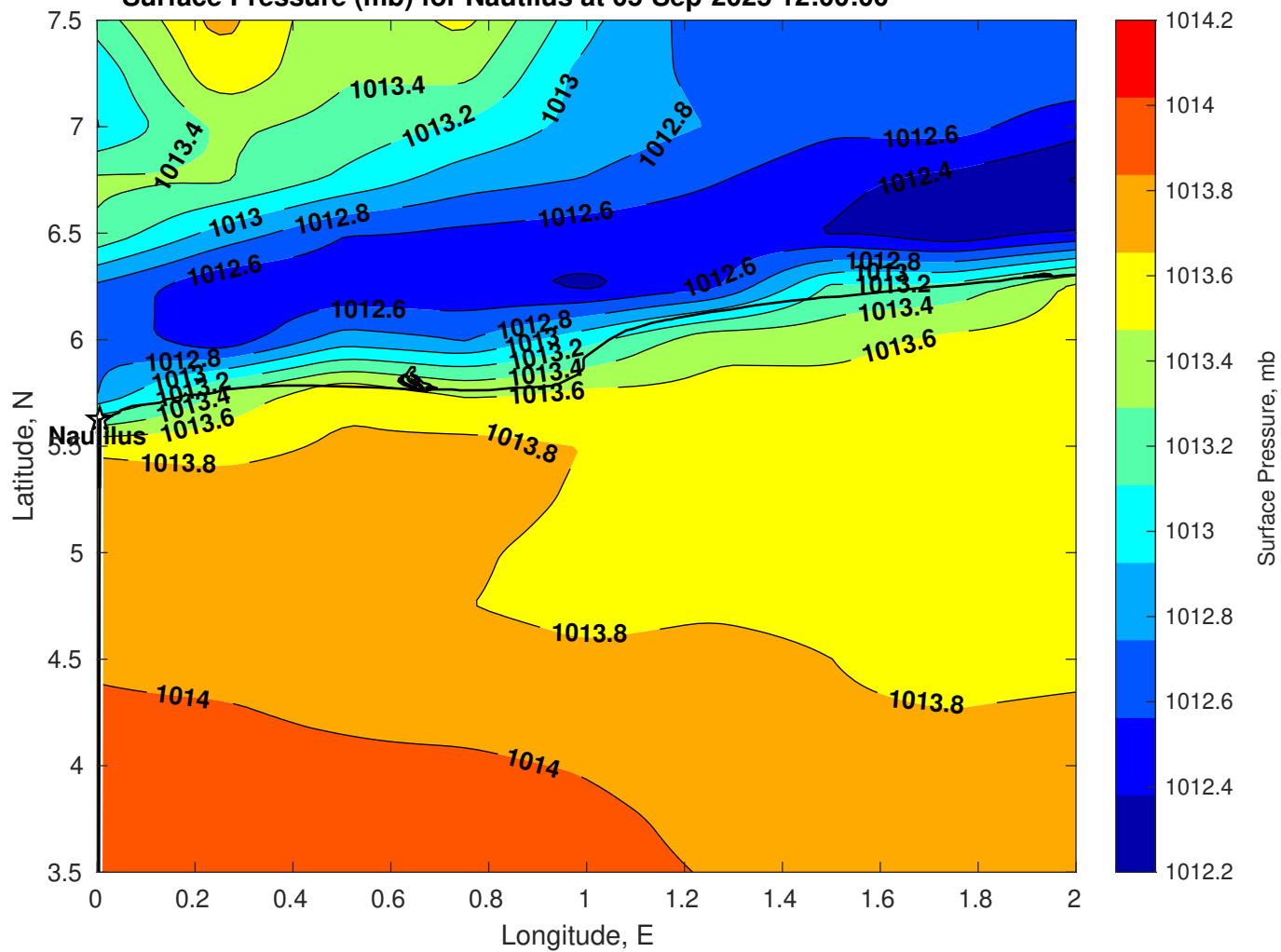
Surface Pressure (mb) for Nautilus at 05-Sep-2025 12:00:00
