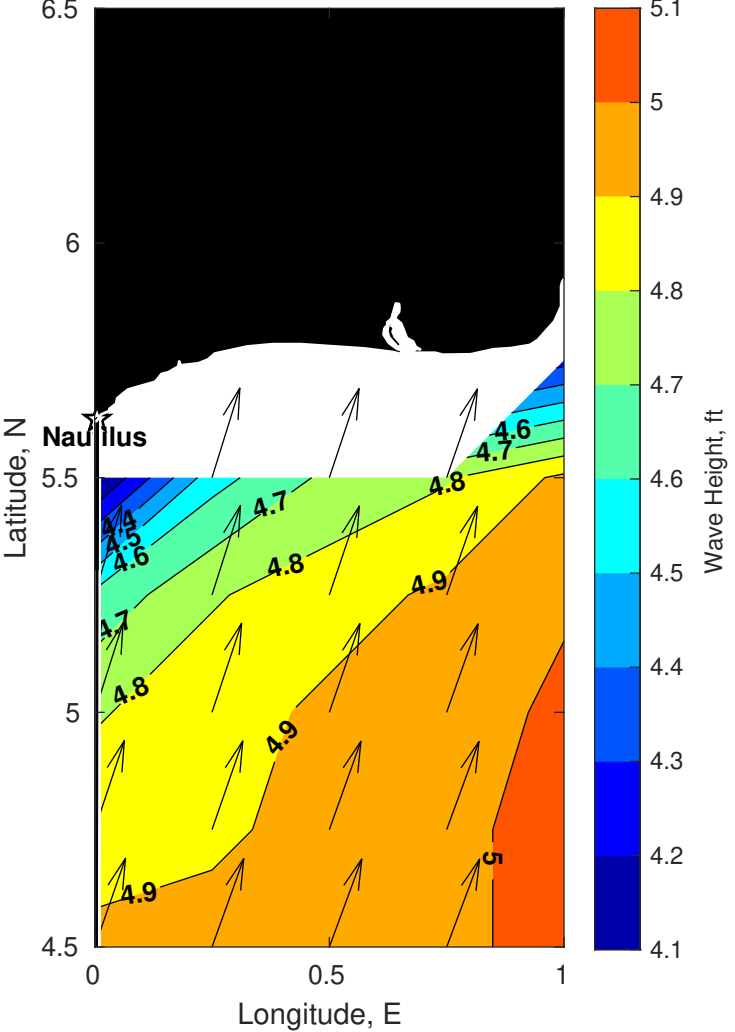
Wave Height (ft) for Nautilus at 04-Sep-2025 21:00:00
