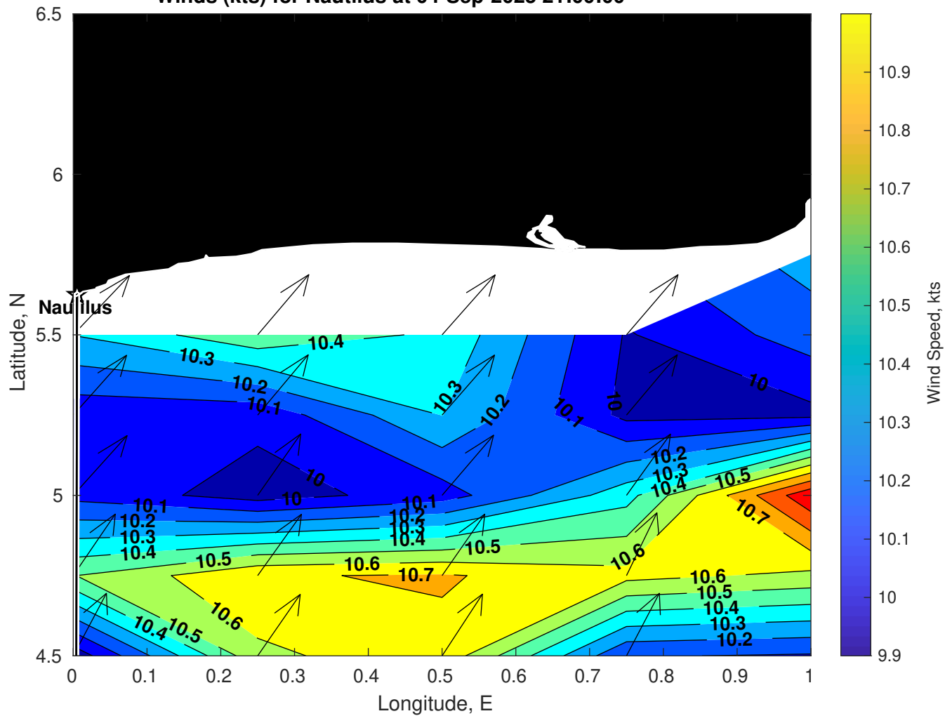
Winds (kts) for Nautilus at 04-Sep-2025 21:00:00
