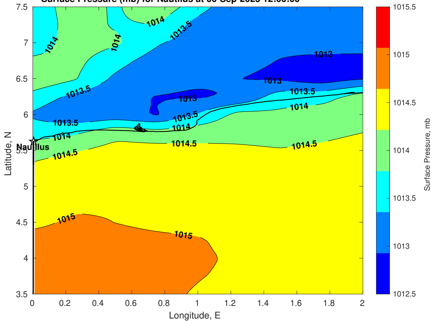
Surface Pressure (mb) for Nautilus at 06-Sep-2025 12:00:00
