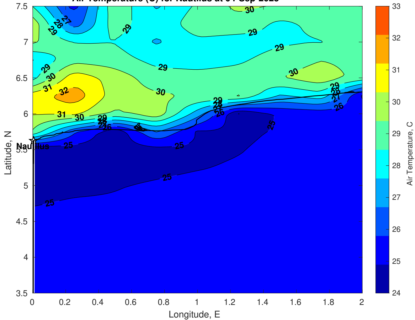
Air Temperature (C) for Nautilus at 04-Sep-2025
