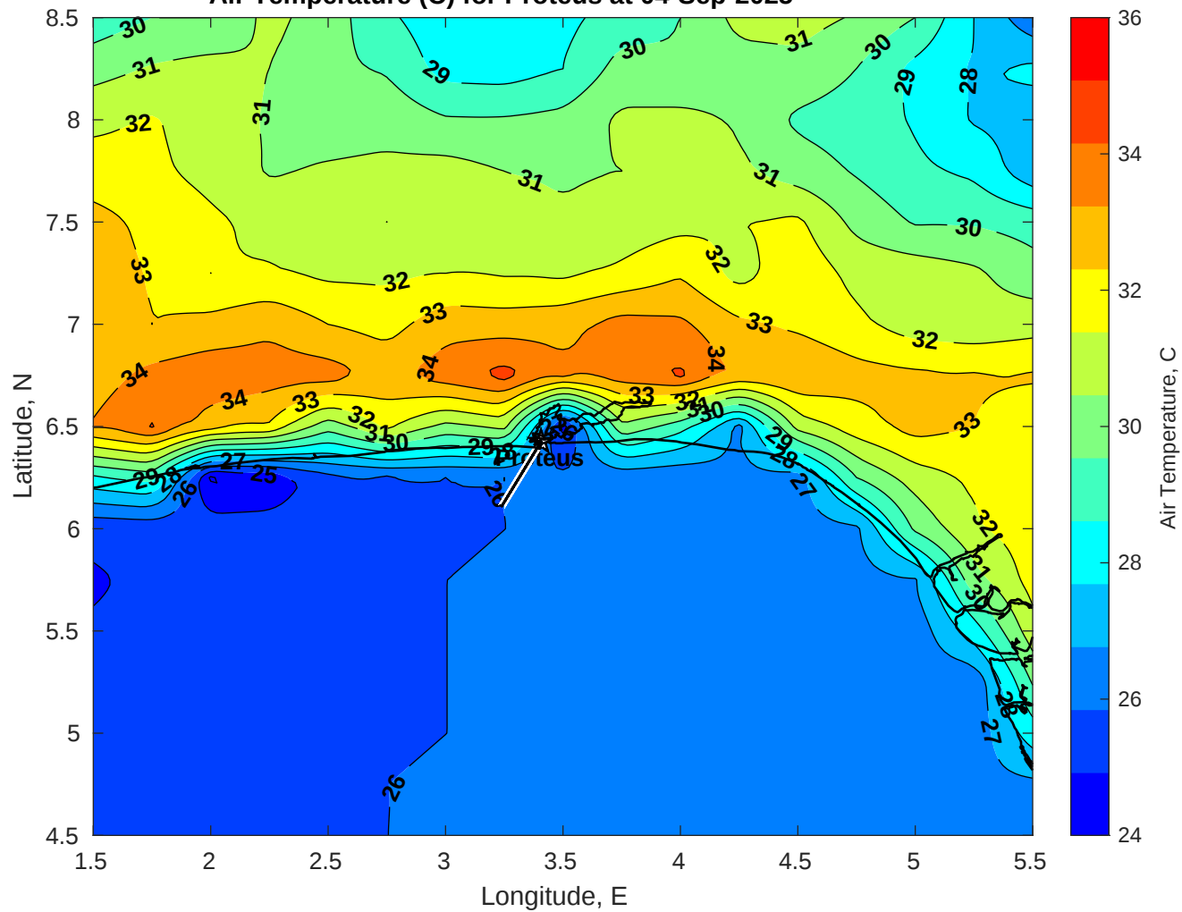
Air Temperature (C) for Proteus at 04-Sep-2025
