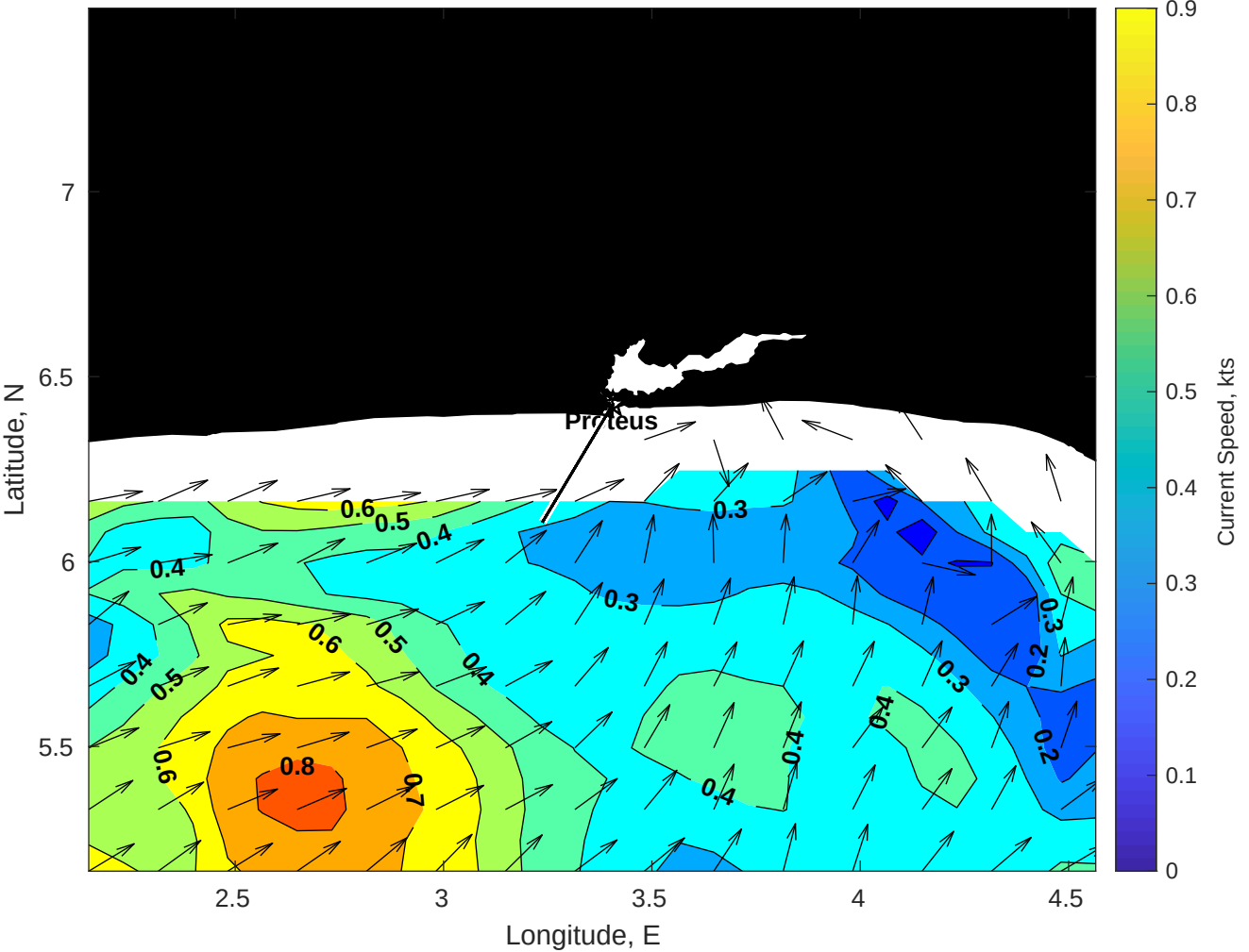
Surface Currents for Proteus at 04-Sep-2025 00:00:00
