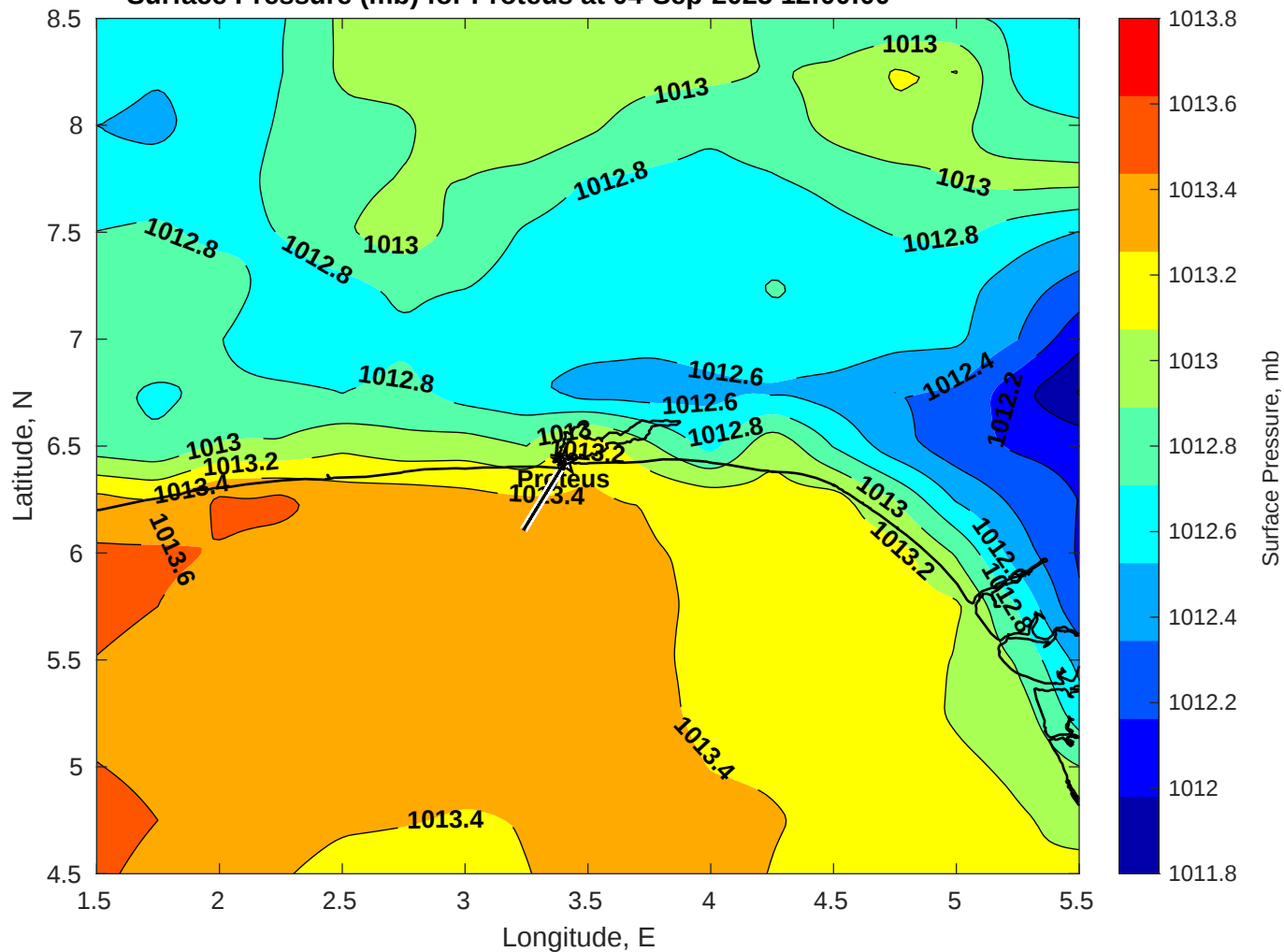
Surface Pressure (mb) for Proteus at 04-Sep-2025 12:00:00
