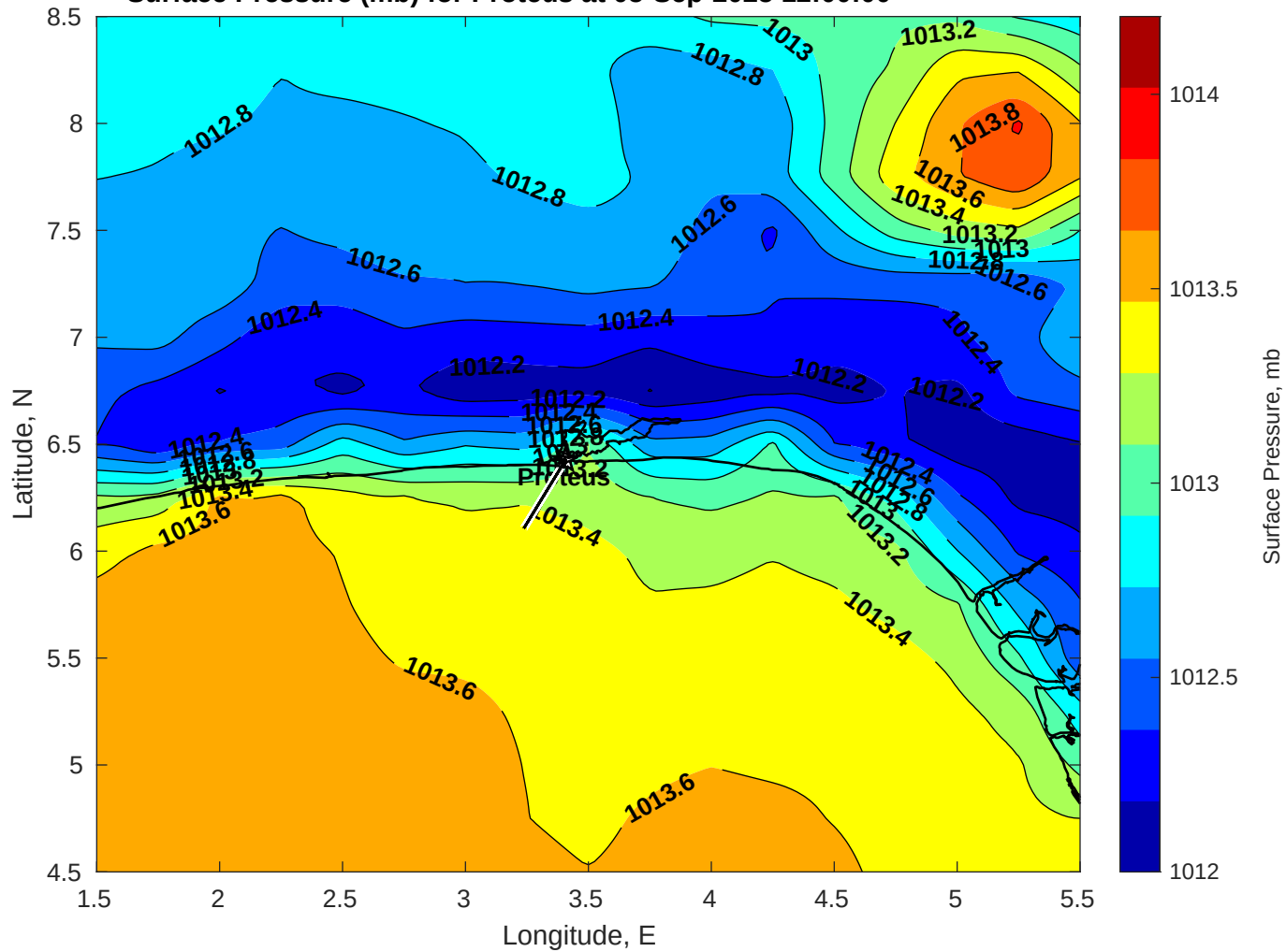
Surface Pressure (mb) for Proteus at 05-Sep-2025 12:00:00
