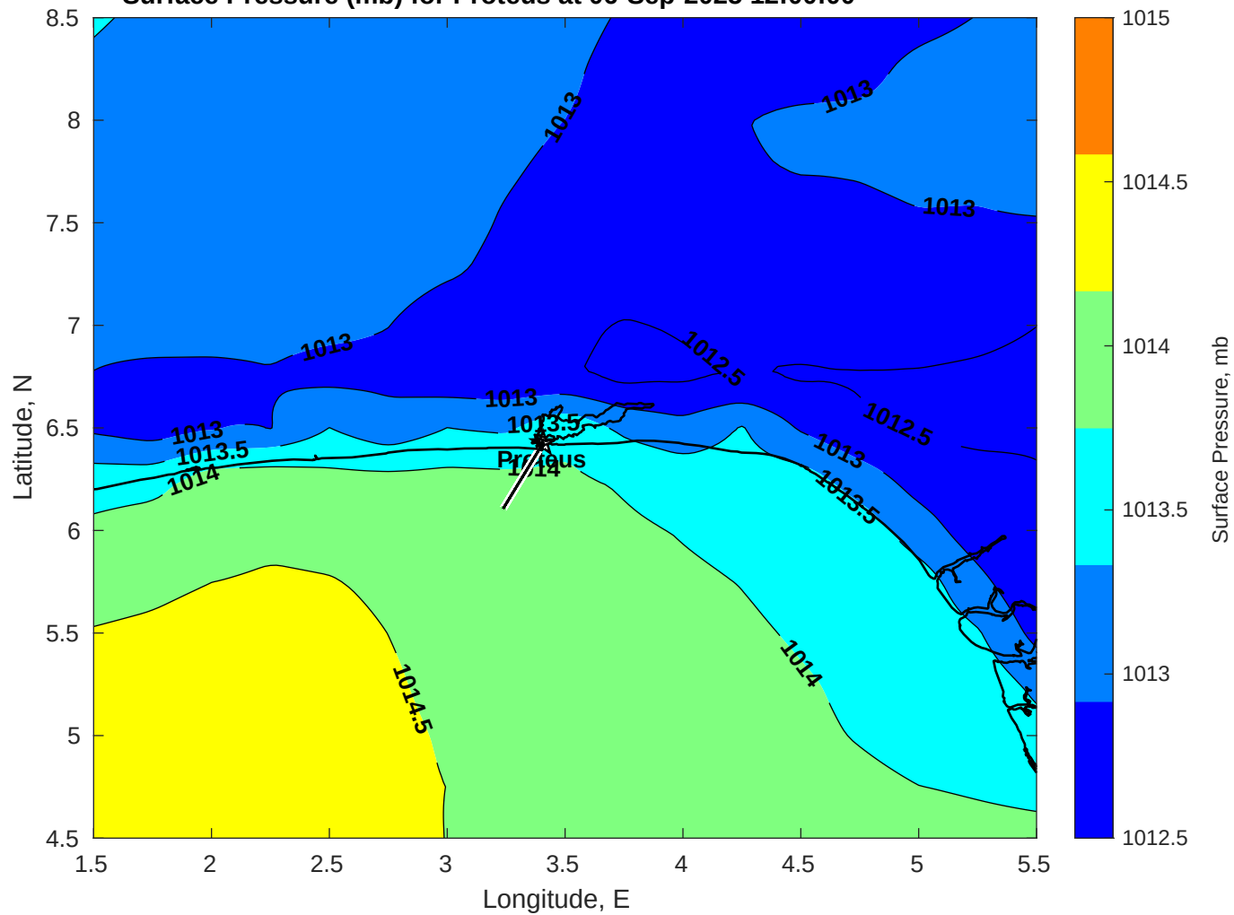
Surface Pressure (mb) for Proteus at 06-Sep-2025 12:00:00
