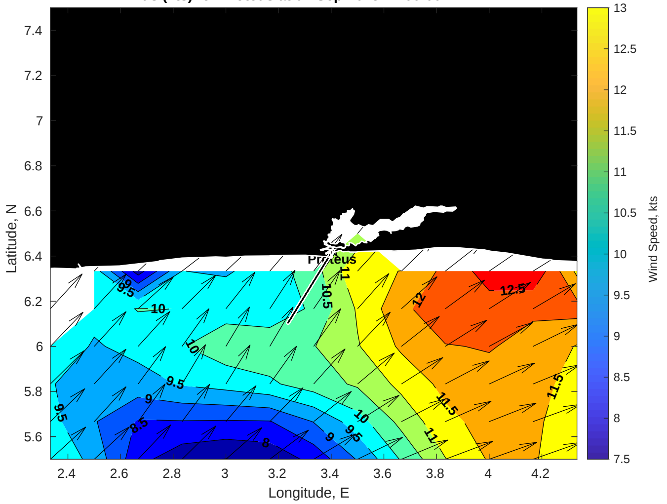
Winds (kts) for Proteus at 04-Sep-2025 21:00:00
