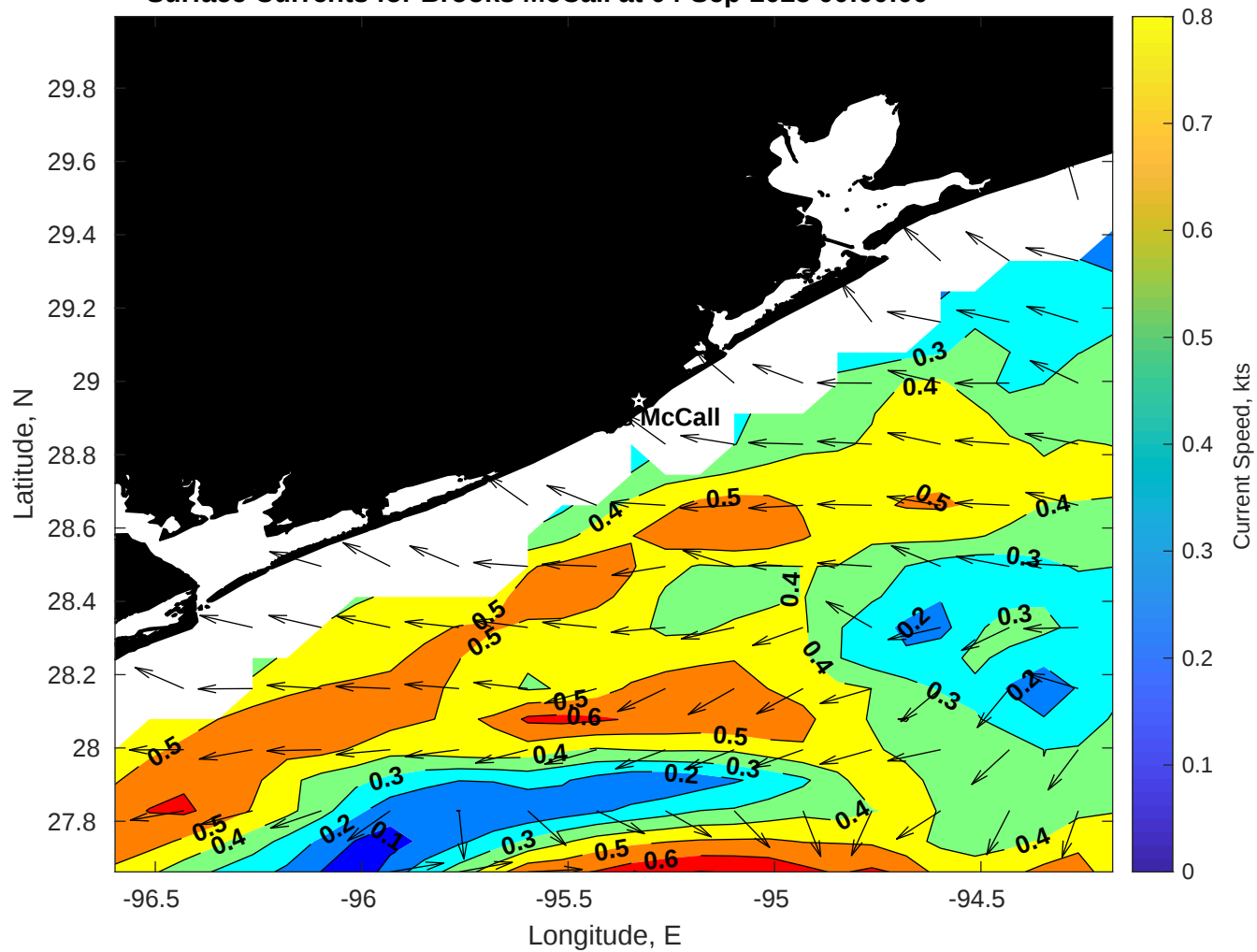
Surface Currents for Brooks McCall at 04-Sep-2025 00:00:00
