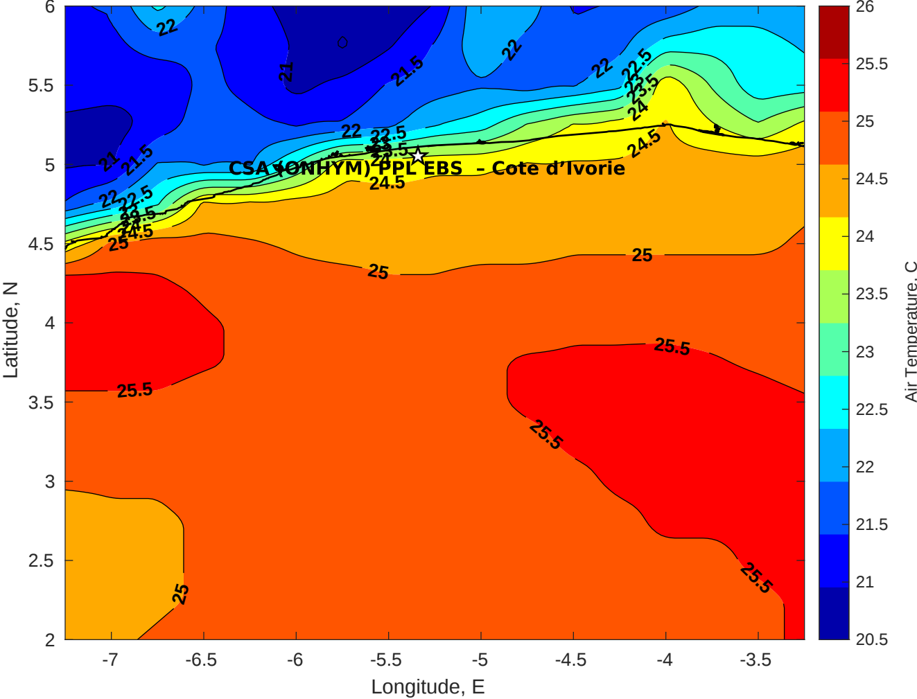
Air Temperature (C) for CSA (ONHYM) PPL EBS - Cote d'Ivoire at 05-Sep-2025
