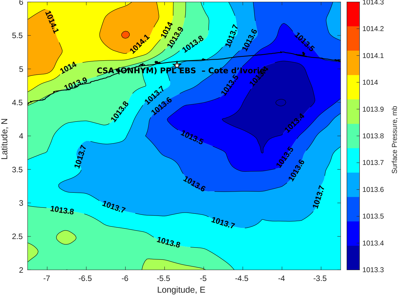
Surface Pressure (mb) for CSA (ONHYM) PPL EBS - Cote d'Ivoire at 05-Sep-2025 00:00:00
