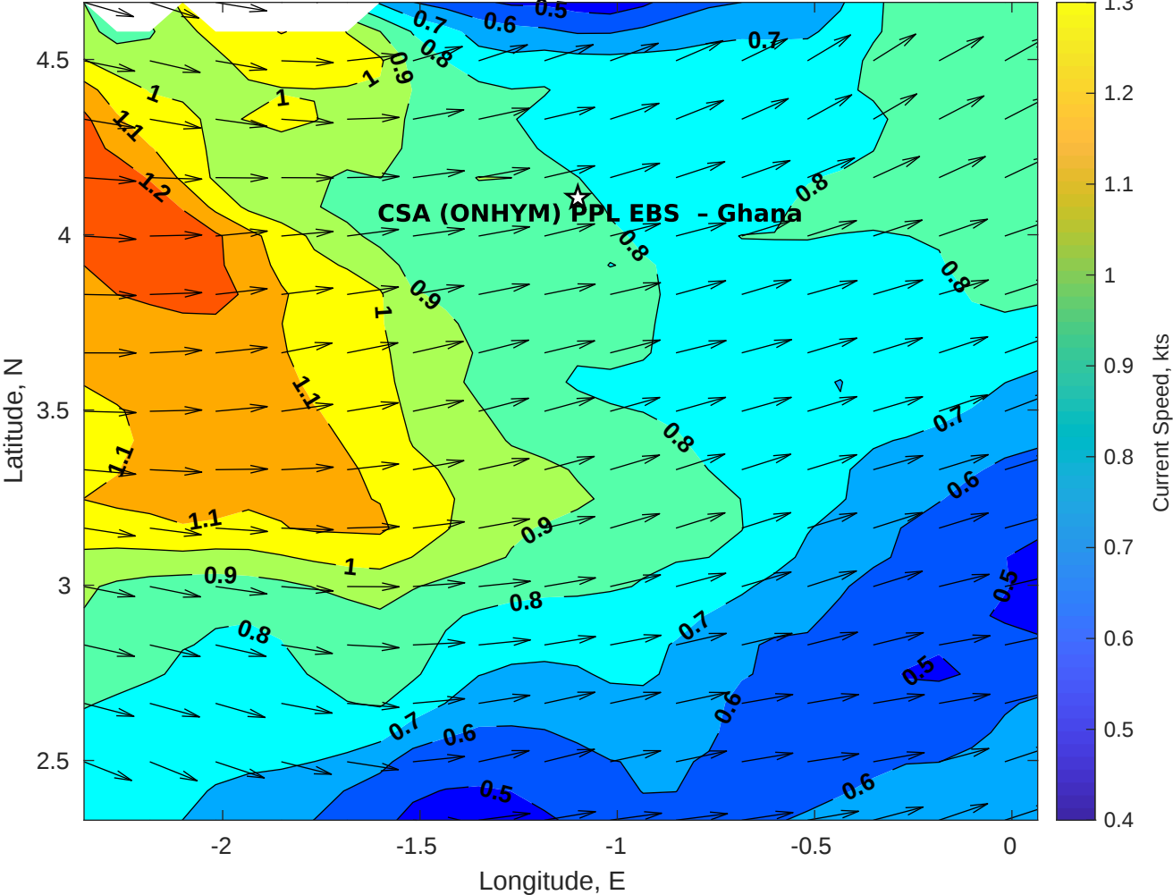
Surface Currents for CSA (ONHYM) PPL EBS - Ghana at 04-Sep-2025 00:00:00
