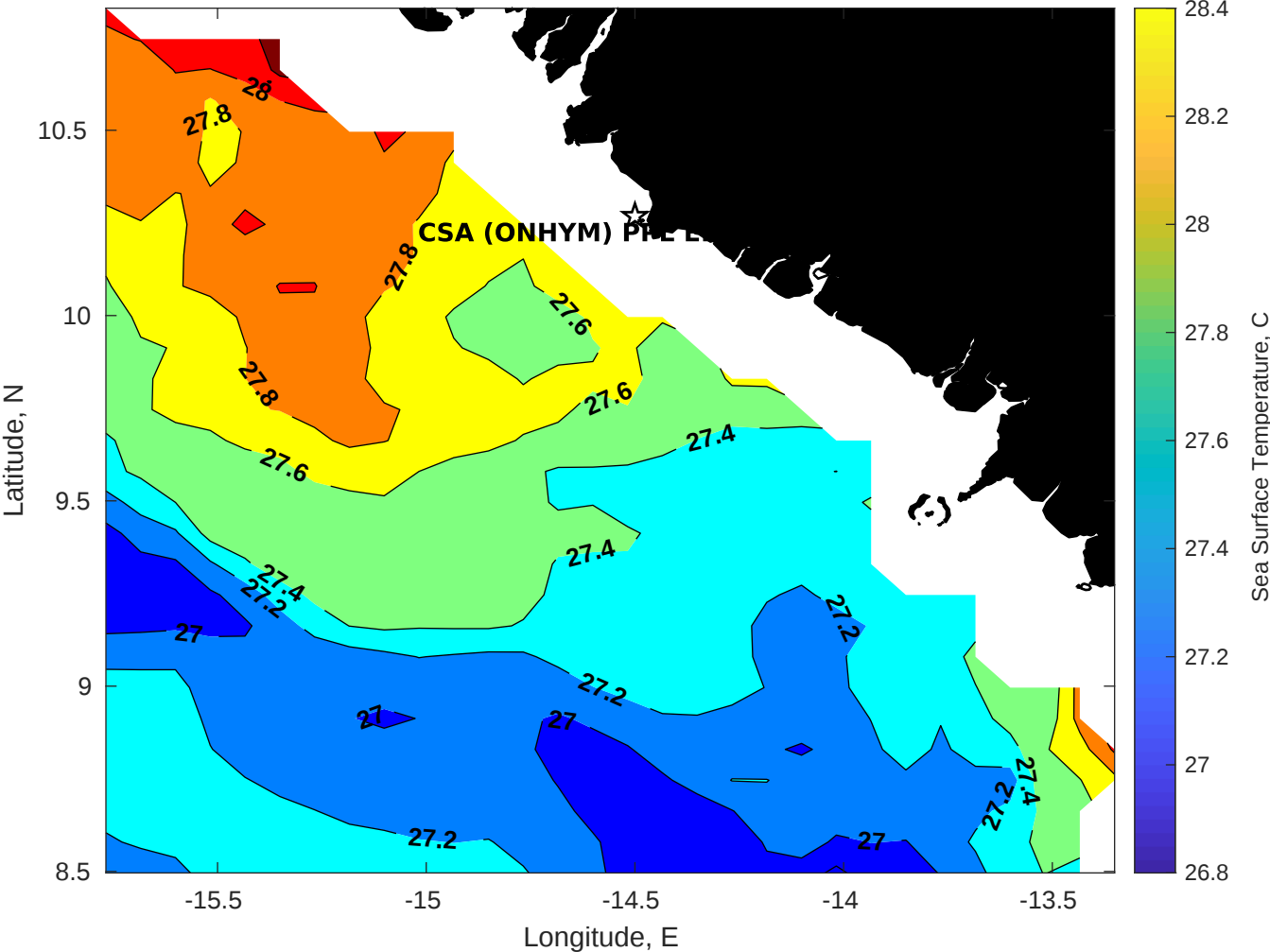
SST for CSA (ONHYM) PPL EBS - Guinea at 04-Sep-2025 00:00:00
