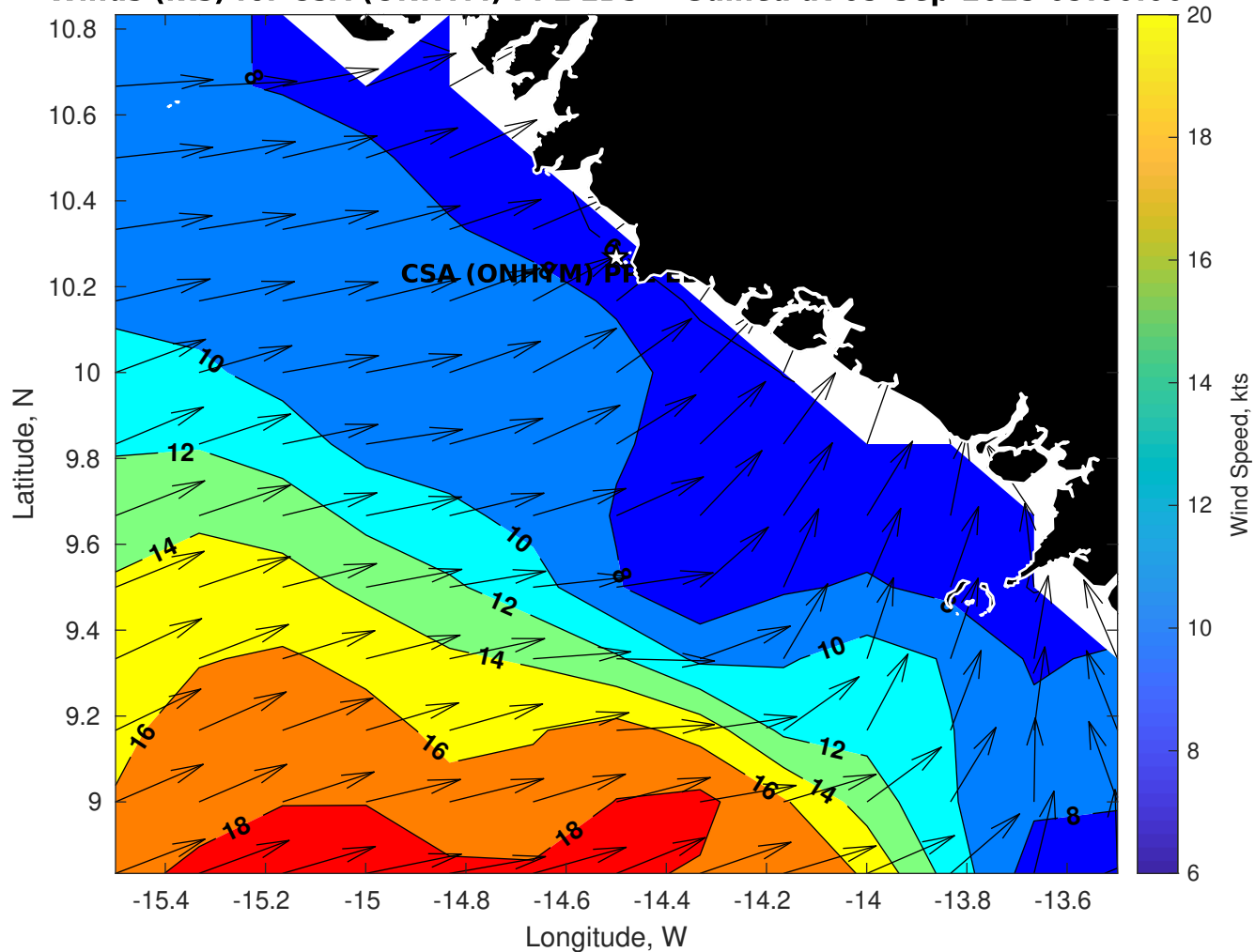
Winds (kts) for CSA (ONHYM) PPL EBS - Guinea at 05-Sep-2025 09:00:00
