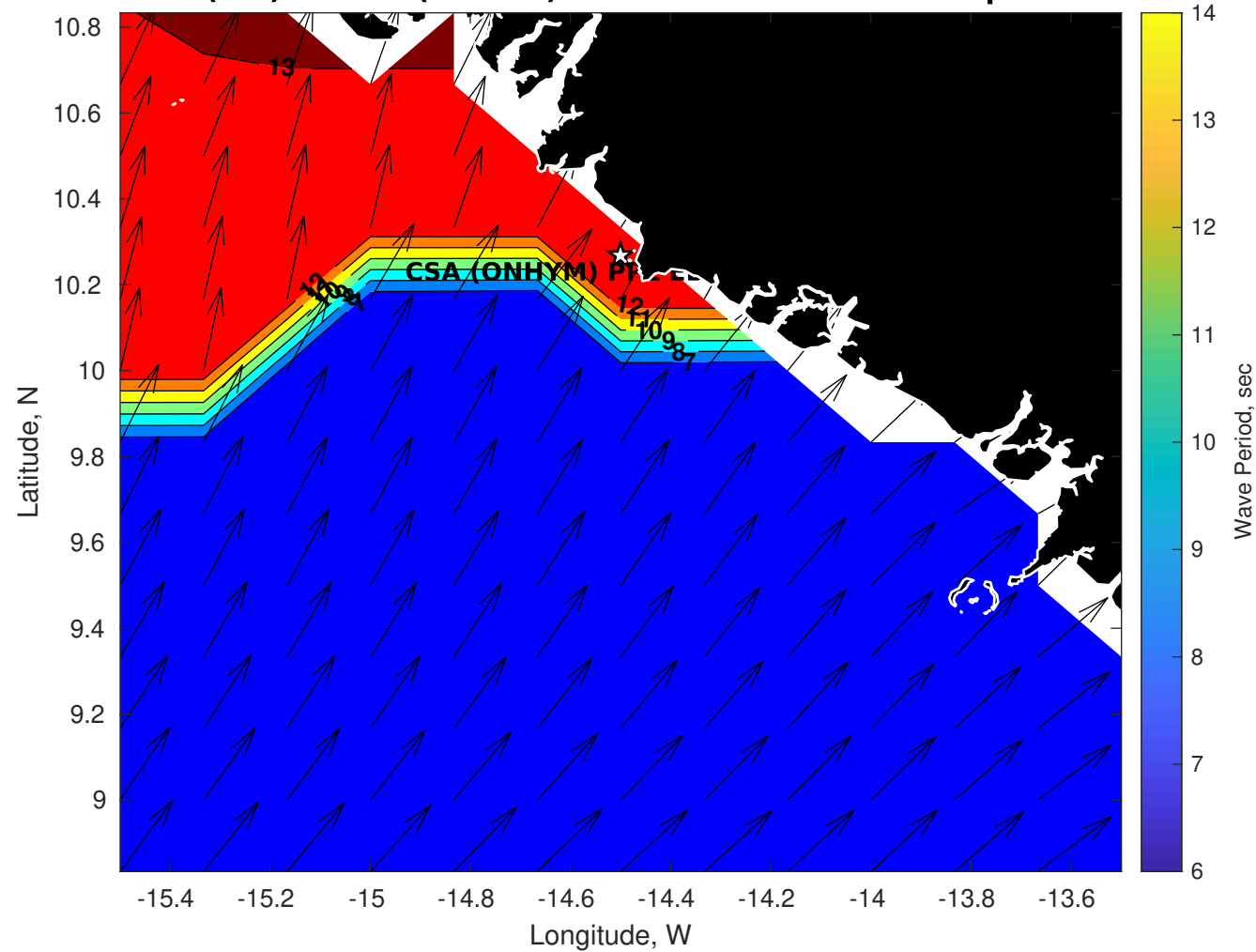
Wave Period (sec) for CSA (ONHYM) PPL EBS - Guinea at 05-Sep-2025 09:00:00
