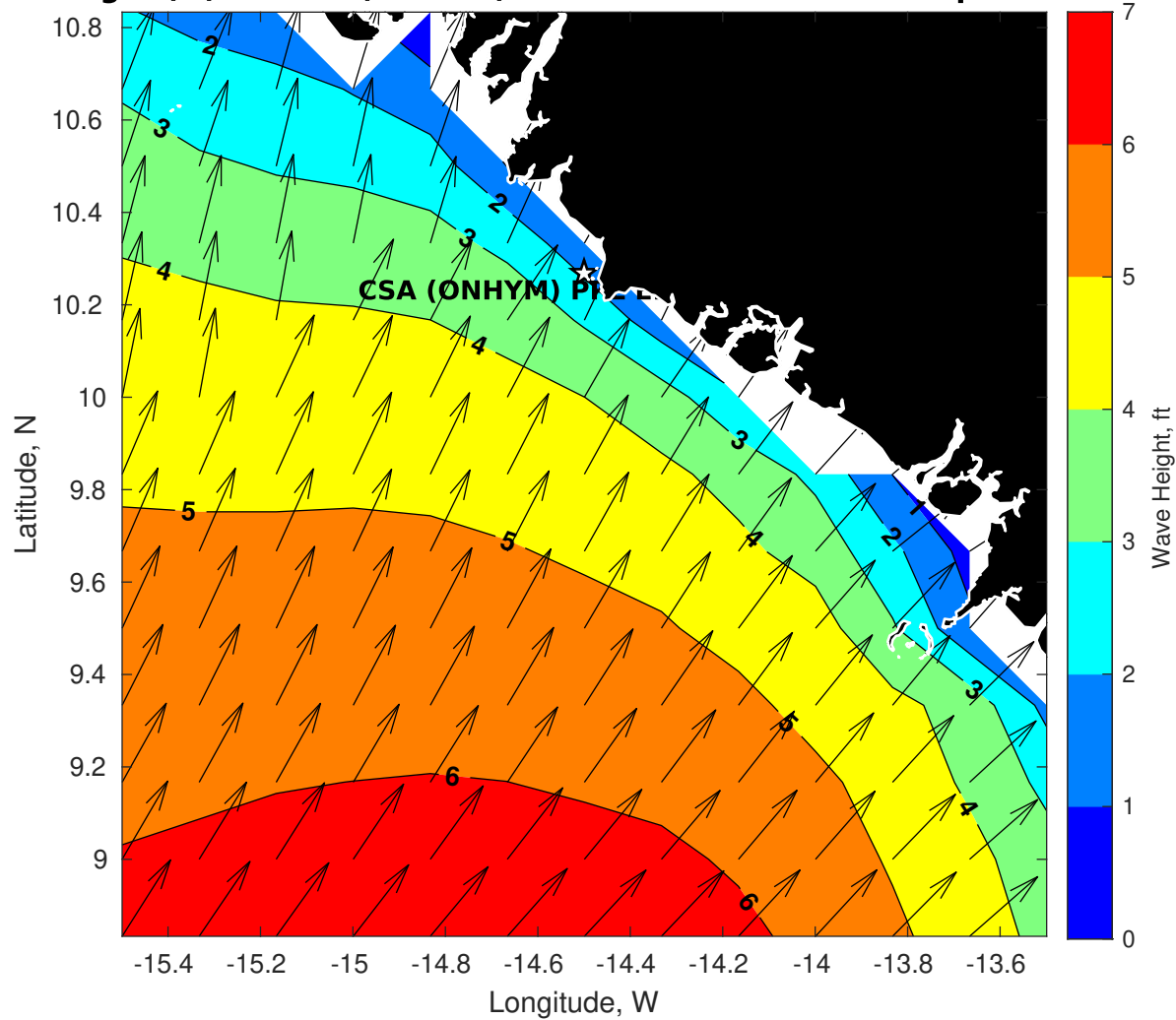
Wave Height (ft) for CSA (ONHYM) PPL EBS - Guinea at 05-Sep-2025 09:00:00
