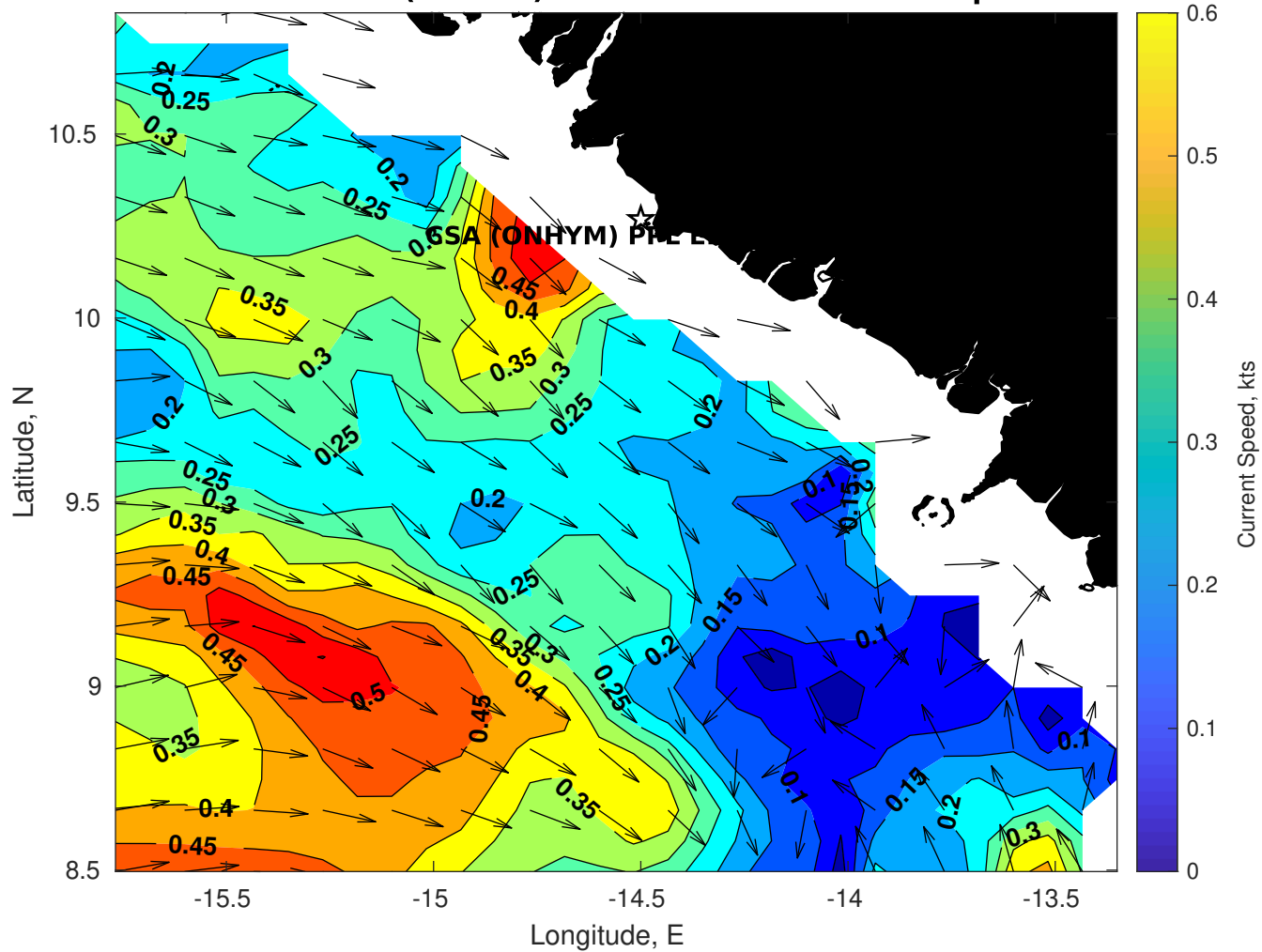
Surface Currents for CSA (ONHYM) PPL EBS - Guinea at 04-Sep-2025 00:00:00
